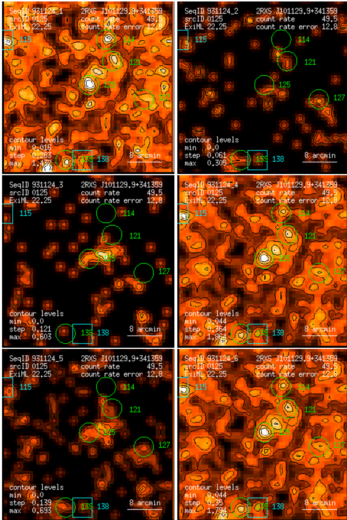
Figure 125: RASS 931124: detection 0125: band rate images, Gaussian filter: (1) PSPC channels 11 – 41, (2) 52 – 90, (3) 91 – 201, (4) 11 – 235, (5) 52 – 201, (6) 11 – 201. Broad band rates in counts/ks. Band rate contour levels in counts/ks/arcmin 2 .
