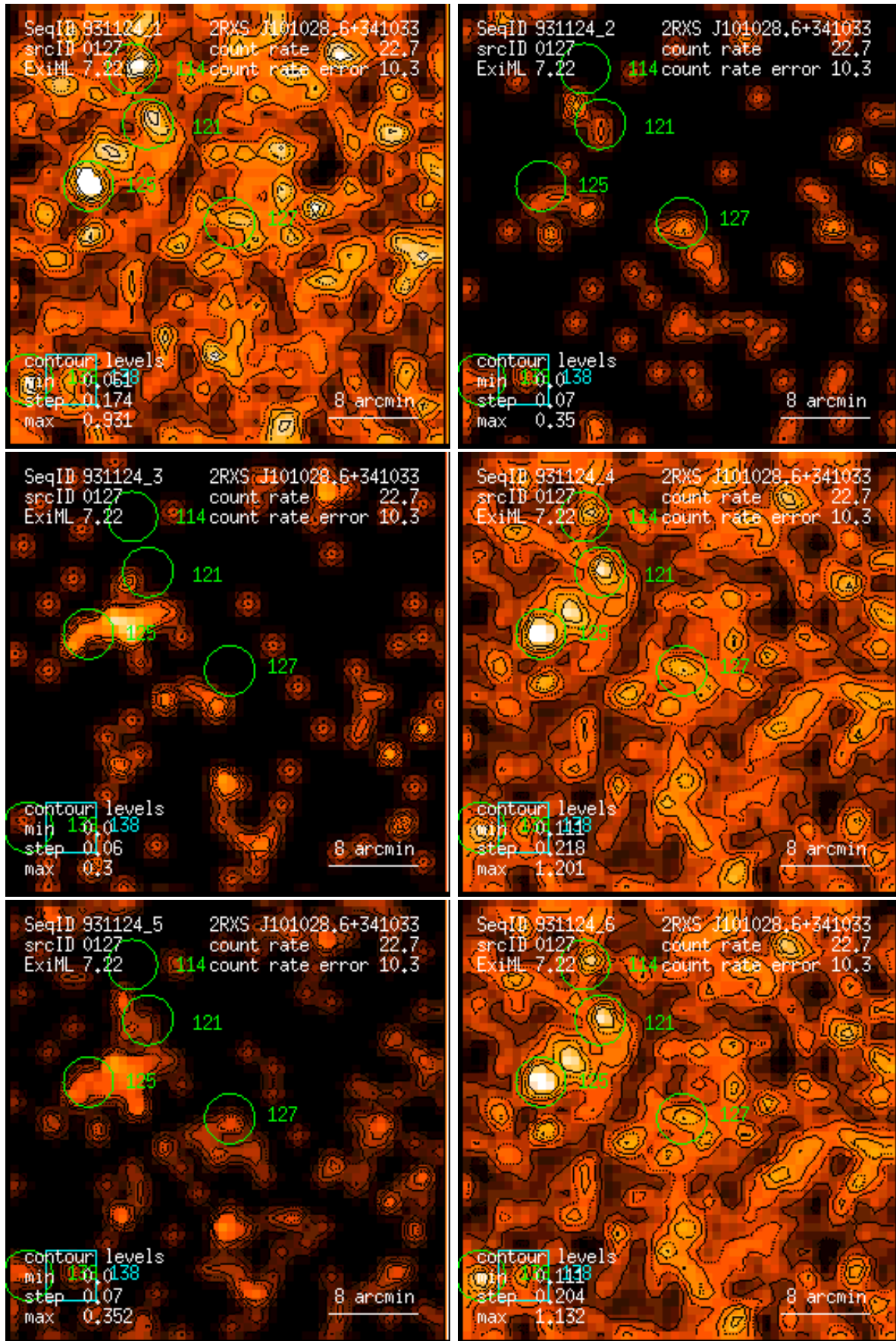
Figure 127: RASS 931124: detection 0127: band rate images, Gaussian filter: (1) PSPC channels 11 – 41, (2) 52 – 90, (3) 91 – 201, (4) 11 – 235, (5) 52 – 201, (6) 11 – 201. Broad band rates in counts/ks. Band rate contour levels in counts/ks/arcmin 2 .
