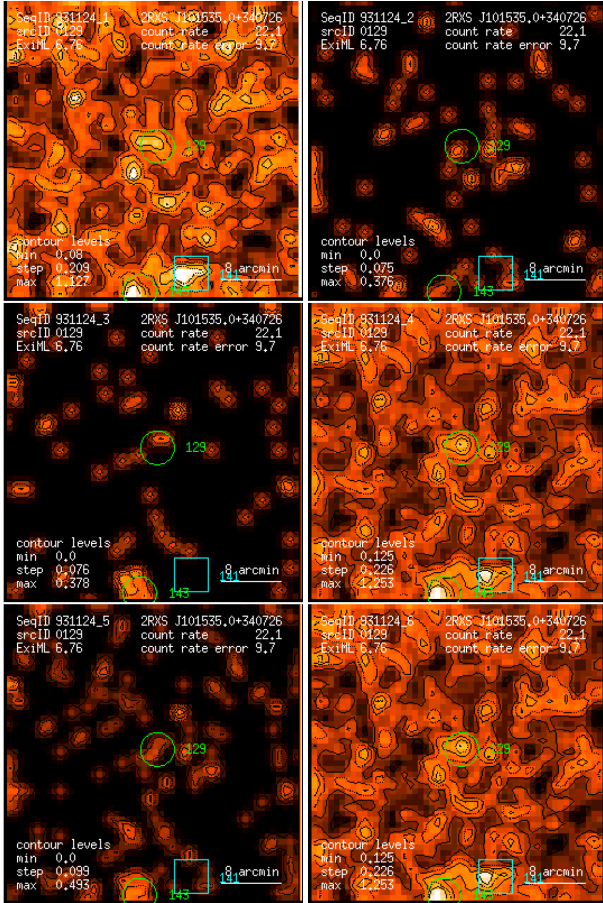
Figure 129: RASS 931124: detection 0129: band rate images, Gaussian filter: (1) PSPC channels 11 – 41, (2) 52 – 90, (3) 91 – 201, (4) 11 – 235, (5) 52 – 201, (6) 11 – 201. Broad band rates in counts/ks. Band rate contour levels in counts/ks/arcmin 2 .
