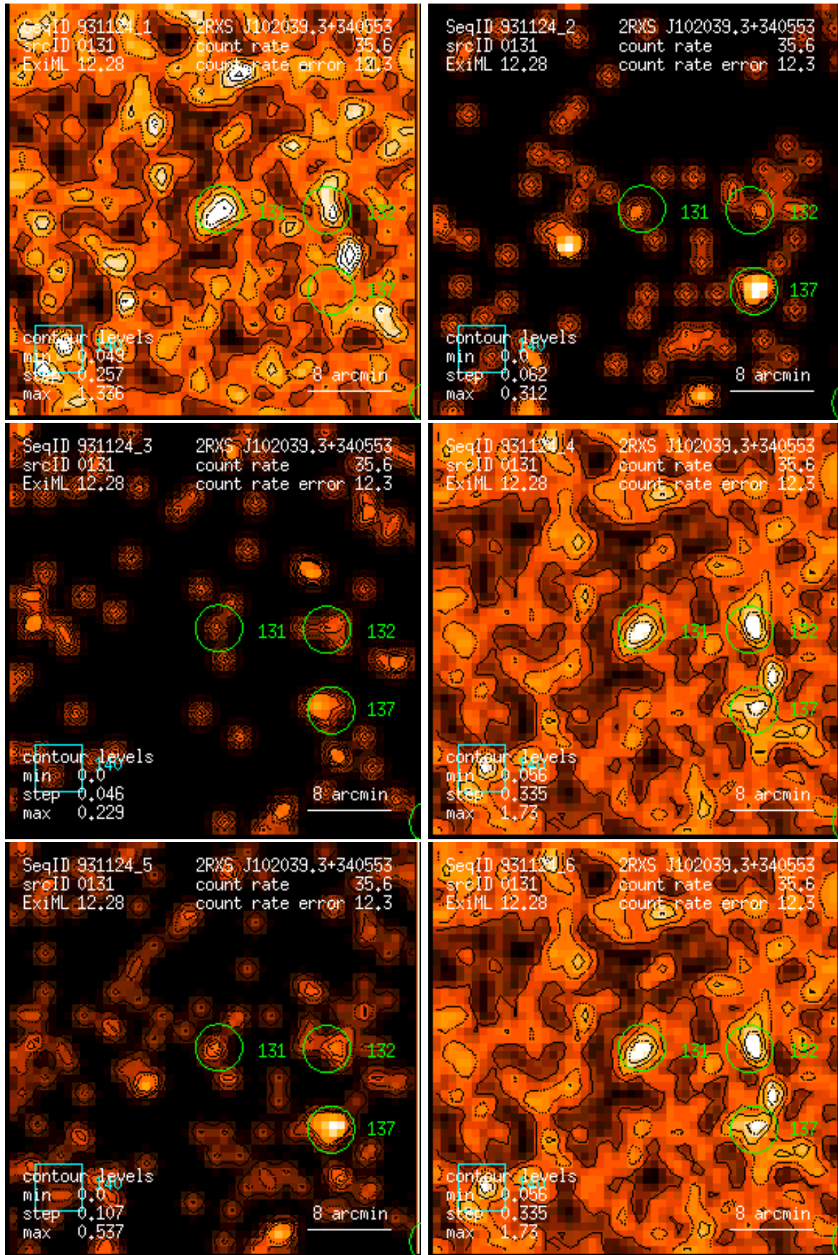
Figure 131: RASS 931124: detection 0131: band rate images, Gaussian filter: (1) PSPC channels 11 – 41, (2) 52 – 90, (3) 91 – 201, (4) 11 – 235, (5) 52 – 201, (6) 11 – 201. Broad band rates in counts/ks. Band rate contour levels in counts/ks/arcmin 2 .
