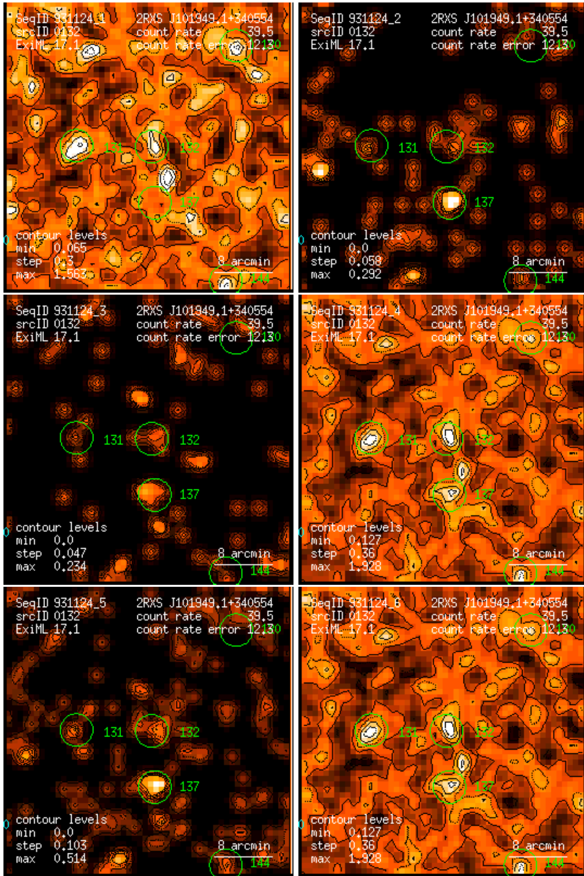
Figure 132: RASS 931124: detection 0132: band rate images, Gaussian filter: (1) PSPC channels 11 – 41, (2) 52 – 90, (3) 91 – 201, (4) 11 – 235, (5) 52 – 201, (6) 11 – 201. Broad band rates in counts/ks. Band rate contour levels in counts/ks/arcmin 2 .
