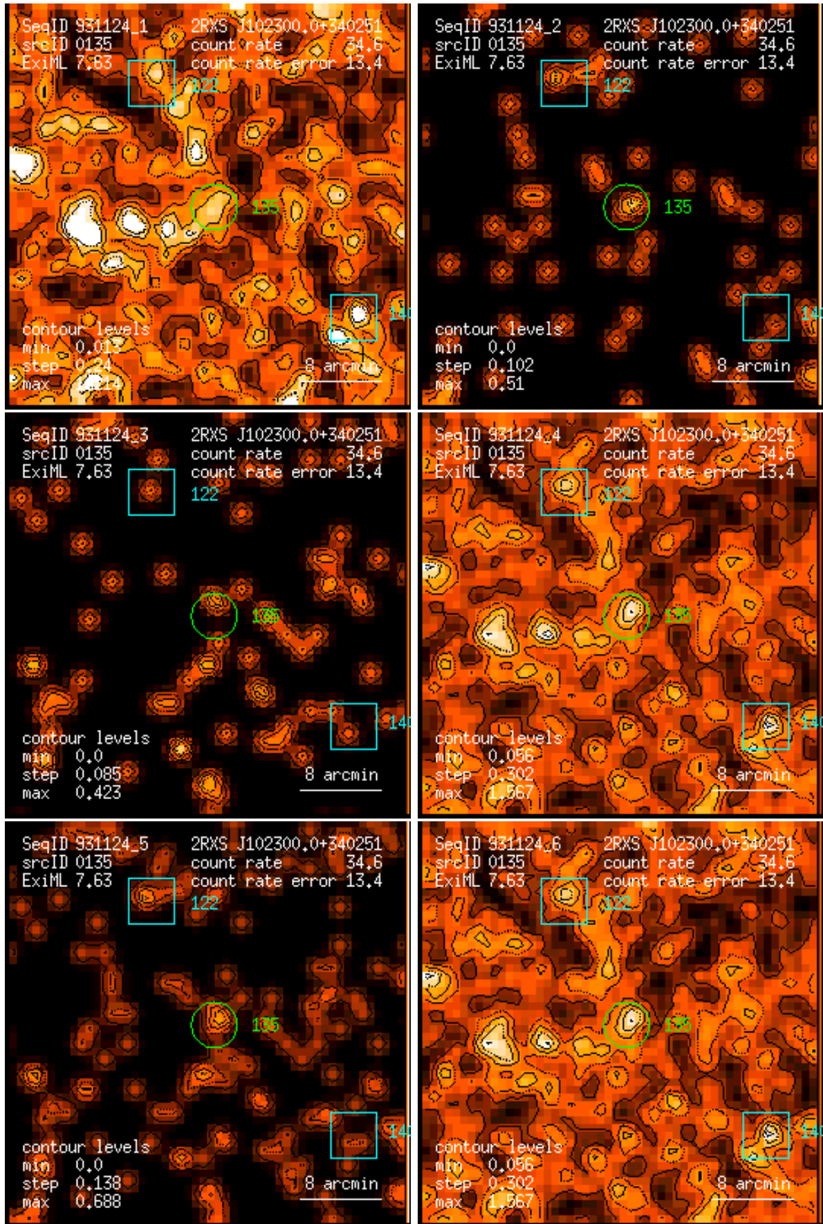
Figure 135: RASS 931124: detection 0135: band rate images, Gaussian filter: (1) PSPC channels 11 – 41, (2) 52 – 90, (3) 91 – 201, (4) 11 – 235, (5) 52 – 201, (6) 11 – 201. Broad band rates in counts/ks. Band rate contour levels in counts/ks/arcmin 2 .
