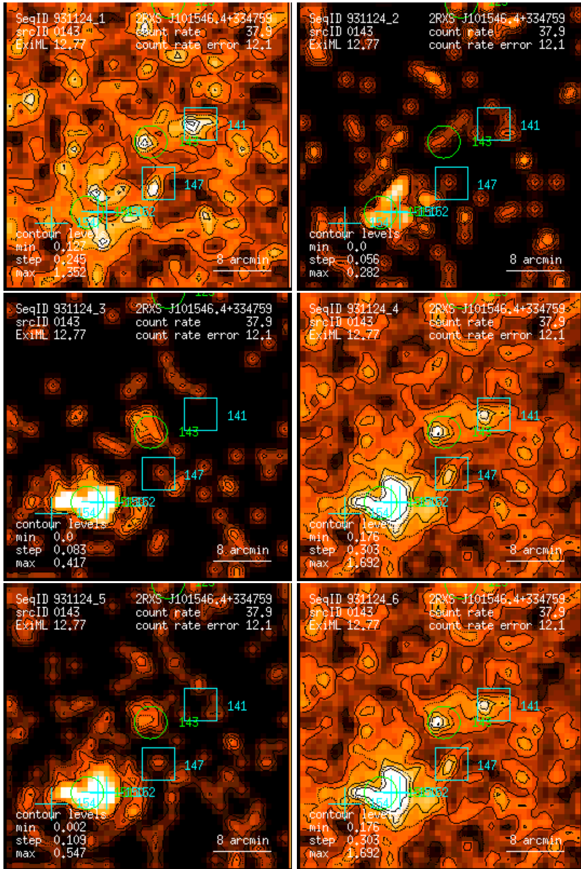
Figure 143: RASS 931124: detection 0143: band rate images, Gaussian filter: (1) PSPC channels 11 – 41, (2) 52 – 90, (3) 91 – 201, (4) 11 – 235, (5) 52 – 201, (6) 11 – 201. Broad band rates in counts/ks. Band rate contour levels in counts/ks/arcmin 2 .
