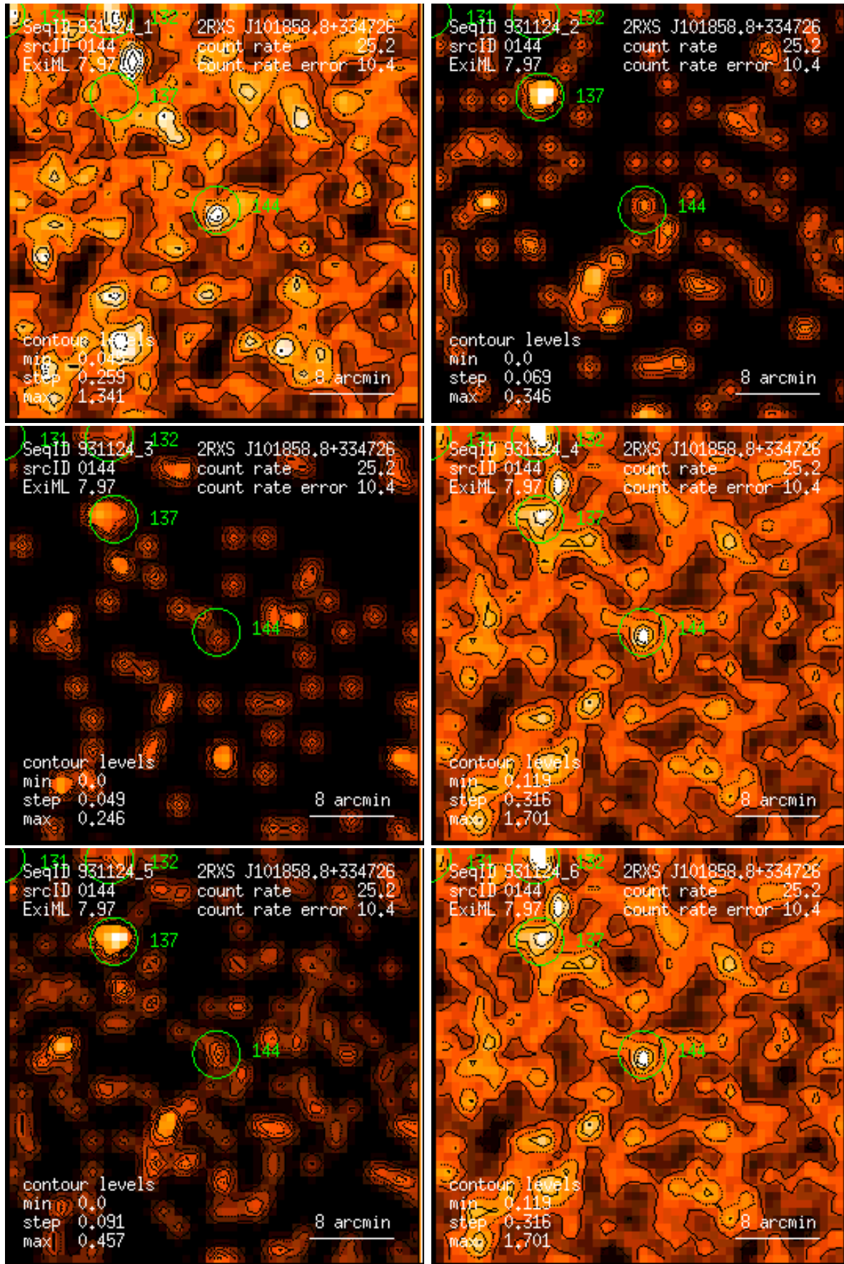
Figure 144: RASS 931124: detection 0144: band rate images, Gaussian filter: (1) PSPC channels 11 – 41, (2) 52 – 90, (3) 91 – 201, (4) 11 – 235, (5) 52 – 201, (6) 11 – 201. Broad band rates in counts/ks. Band rate contour levels in counts/ks/arcmin 2 .
