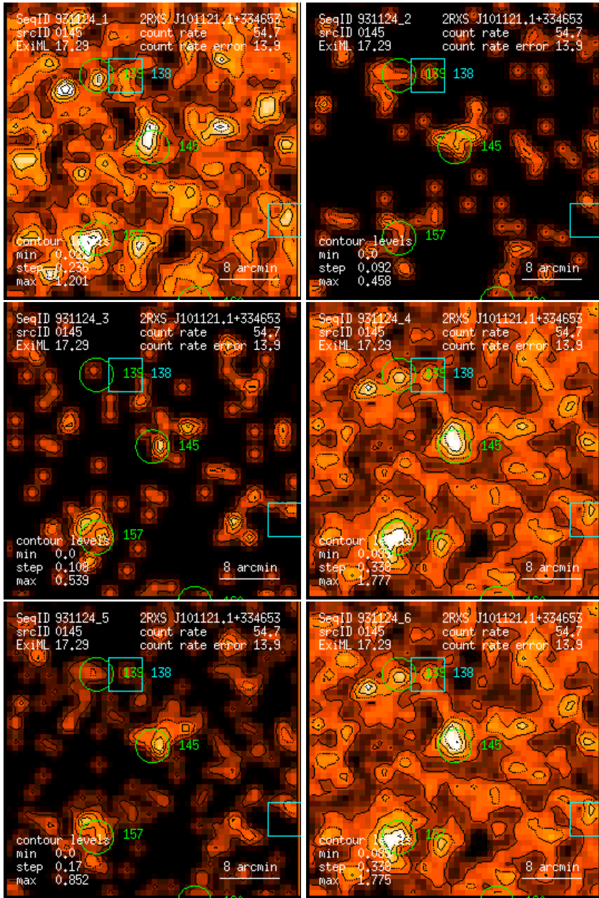
Figure 145: RASS 931124: detection 0145: band rate images, Gaussian filter: (1) PSPC channels 11 – 41, (2) 52 – 90, (3) 91 – 201, (4) 11 – 235, (5) 52 – 201, (6) 11 – 201. Broad band rates in counts/ks. Band rate contour levels in counts/ks/arcmin 2 .
