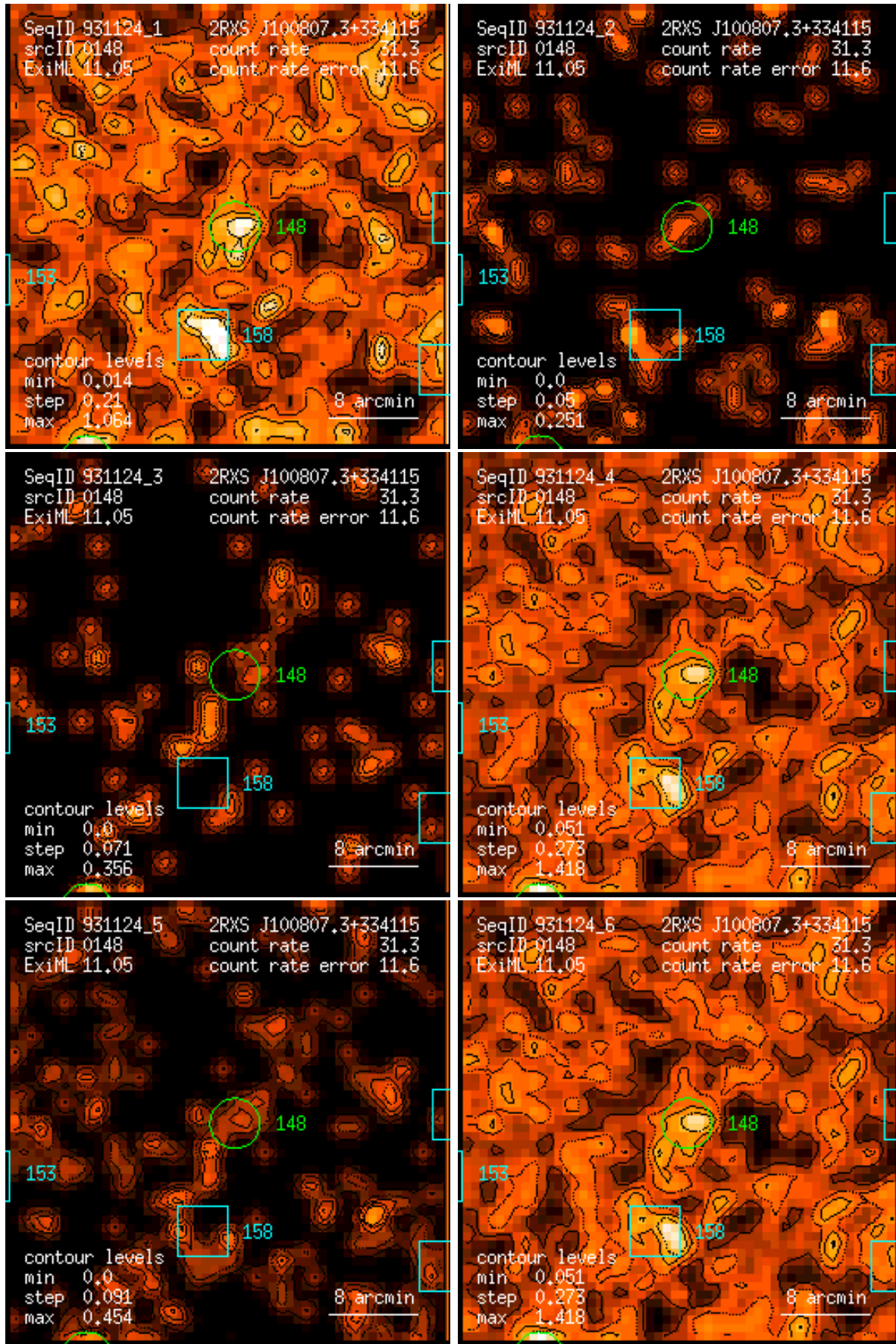
Figure 148: RASS 931124: detection 0148: band rate images, Gaussian filter: (1) PSPC channels 11 – 41, (2) 52 – 90, (3) 91 – 201, (4) 11 – 235, (5) 52 – 201, (6) 11 – 201. Broad band rates in counts/ks. Band rate contour levels in counts/ks/arcmin 2 .
