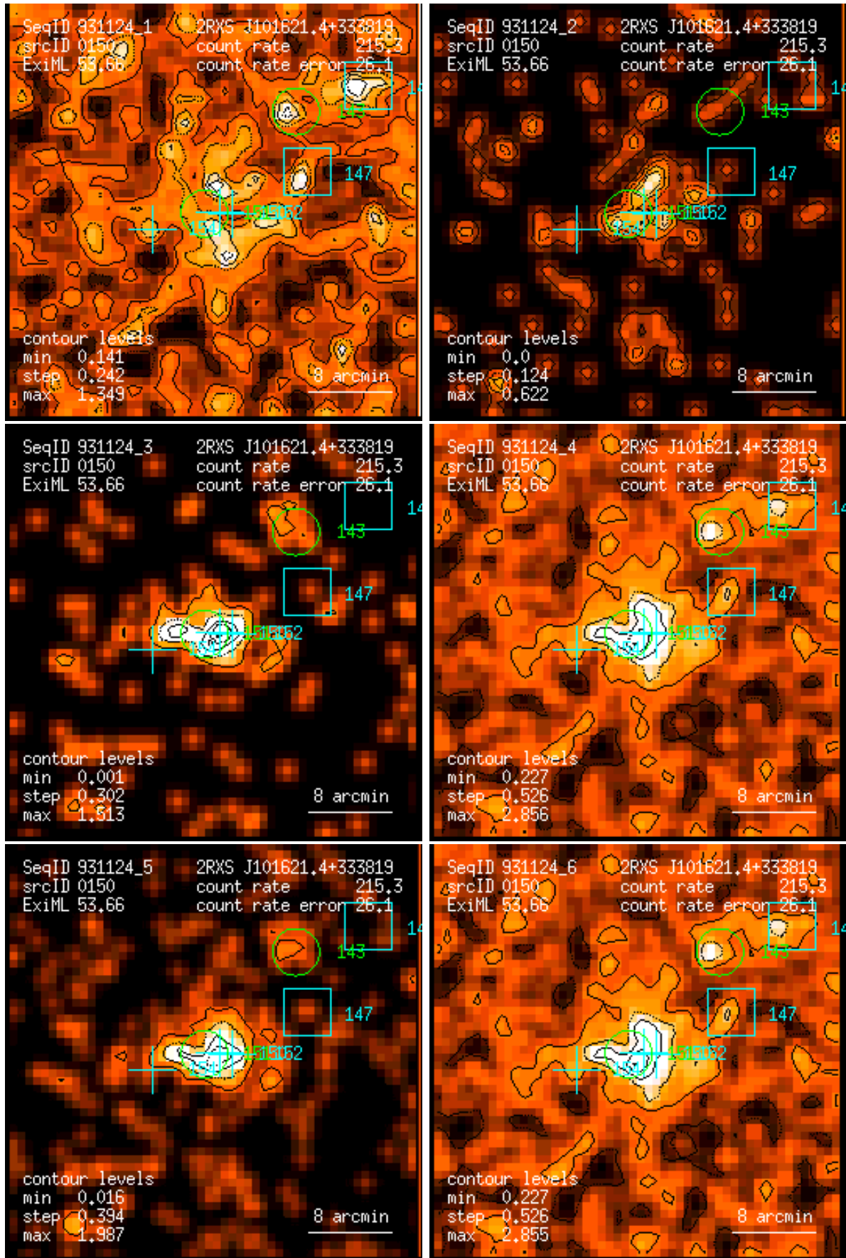
Figure 150: RASS 931124: detection 0150: band rate images, Gaussian filter: (1) PSPC channels 11 – 41, (2) 52 – 90, (3) 91 – 201, (4) 11 – 235, (5) 52 – 201, (6) 11 – 201. Broad band rates in counts/ks. Band rate contour levels in counts/ks/arcmin 2 .
