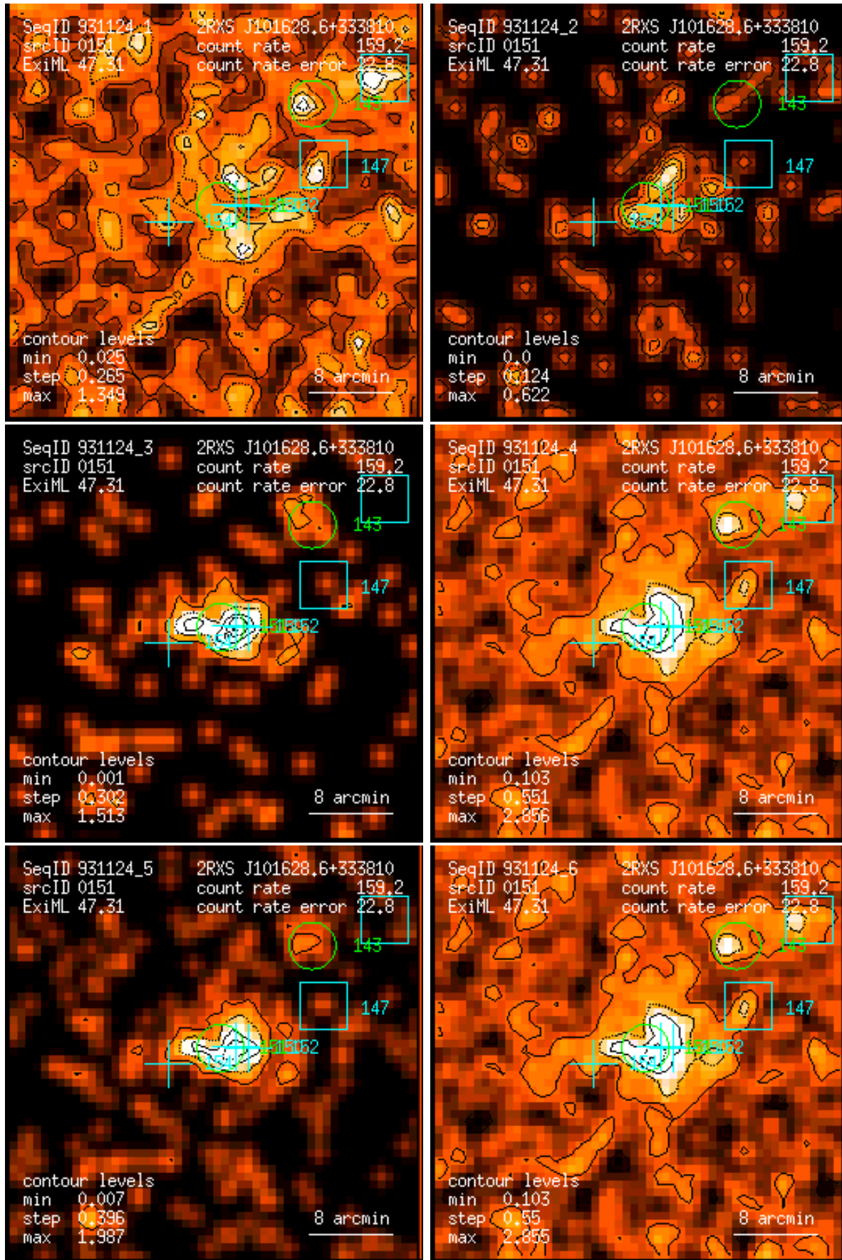
Figure 151: RASS 931124: detection 0151: band rate images, Gaussian filter: (1) PSPC channels 11 – 41, (2) 52 – 90, (3) 91 – 201, (4) 11 – 235, (5) 52 – 201, (6) 11 – 201. Broad band rates in counts/ks. Band rate contour levels in counts/ks/arcmin 2 .
