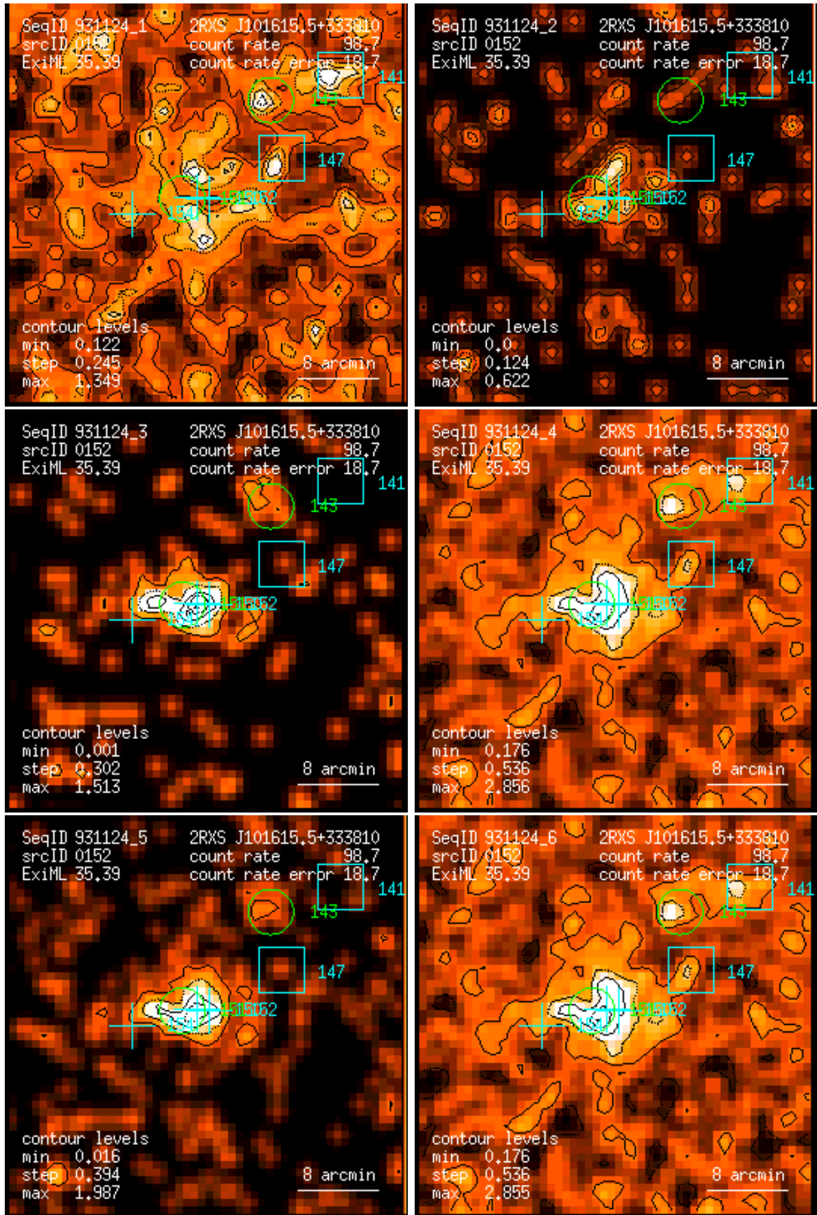
Figure 152: RASS 931124: detection 0152: band rate images, Gaussian filter: (1) PSPC channels 11 – 41, (2) 52 – 90, (3) 91 – 201, (4) 11 – 235, (5) 52 – 201, (6) 11 – 201. Broad band rates in counts/ks. Band rate contour levels in counts/ks/arcmin 2 .
