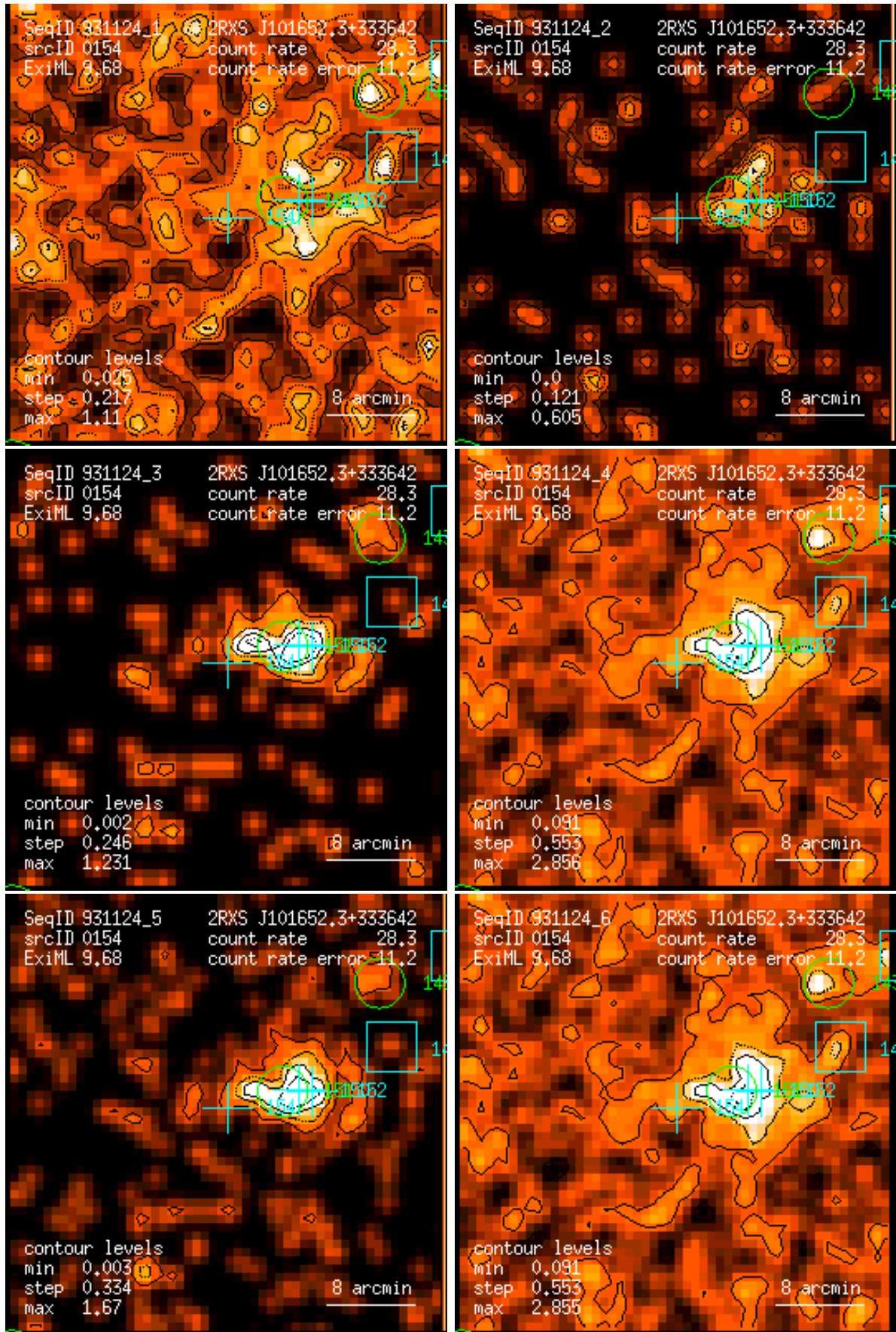
Figure 154: RASS 931124: detection 0154: band rate images, Gaussian filter: (1) PSPC channels 11 – 41, (2) 52 – 90, (3) 91 – 201, (4) 11 – 235, (5) 52 – 201, (6) 11 – 201. Broad band rates in counts/ks. Band rate contour levels in counts/ks/arcmin 2 .
