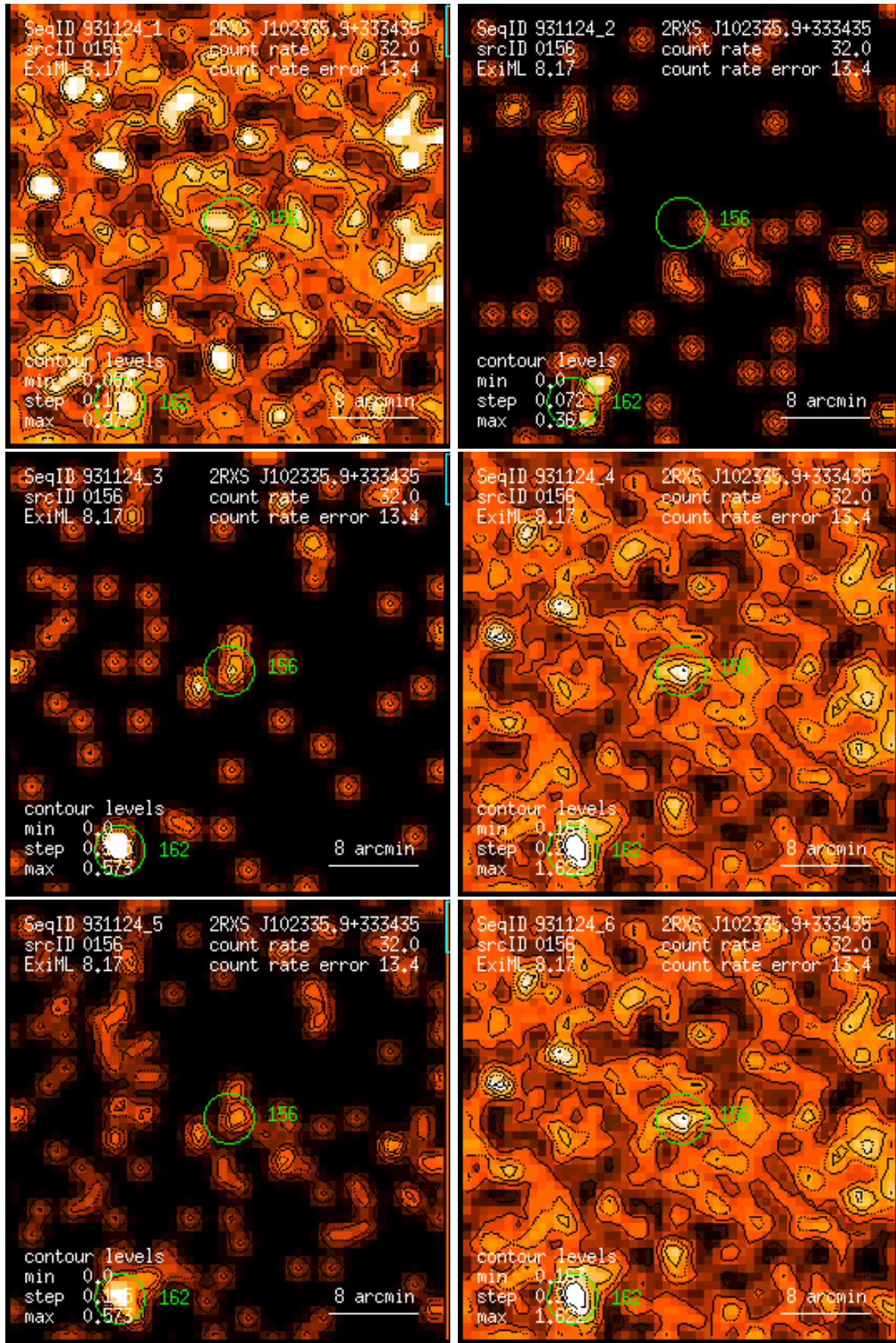
Figure 156: RASS 931124: detection 0156: band rate images, Gaussian filter: (1) PSPC channels 11 – 41, (2) 52 – 90, (3) 91 – 201, (4) 11 – 235, (5) 52 – 201, (6) 11 – 201. Broad band rates in counts/ks. Band rate contour levels in counts/ks/arcmin 2 .
