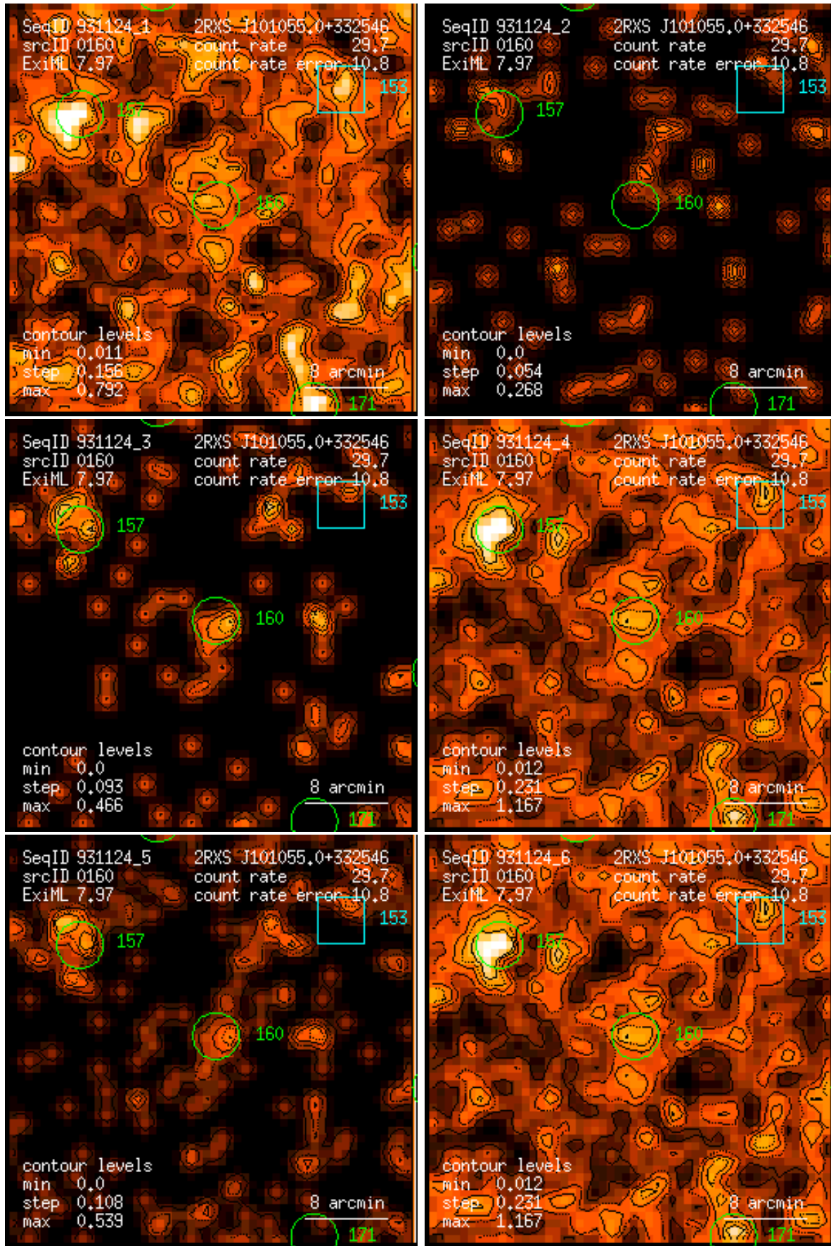
Figure 160: RASS 931124: detection 0160: band rate images, Gaussian filter: (1) PSPC channels 11 – 41, (2) 52 – 90, (3) 91 – 201, (4) 11 – 235, (5) 52 – 201, (6) 11 – 201. Broad band rates in counts/ks. Band rate contour levels in counts/ks/arcmin 2 .
