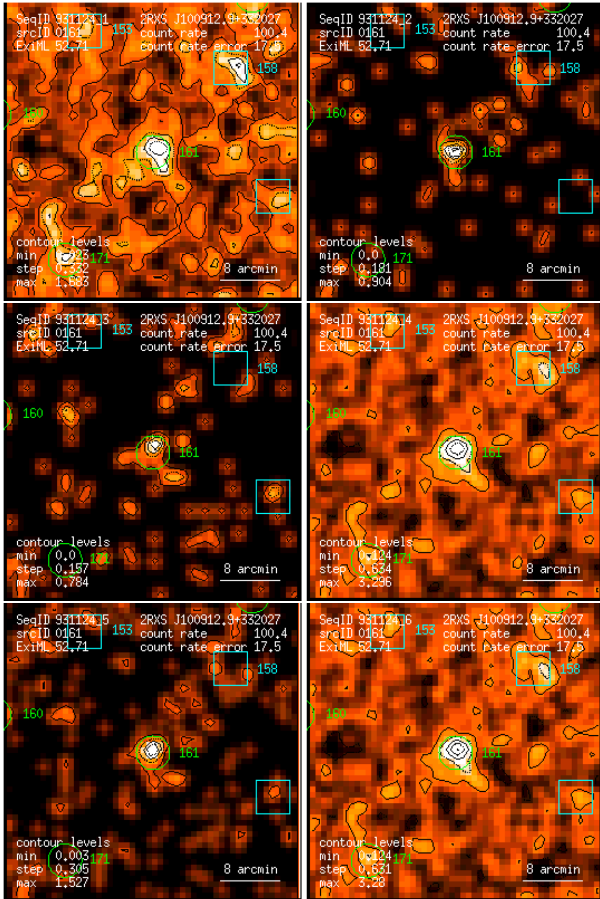
Figure 161: RASS 931124: detection 0161: band rate images, Gaussian filter: (1) PSPC channels 11 – 41, (2) 52 – 90, (3) 91 – 201, (4) 11 – 235, (5) 52 – 201, (6) 11 – 201. Broad band rates in counts/ks. Band rate contour levels in counts/ks/arcmin 2 .
