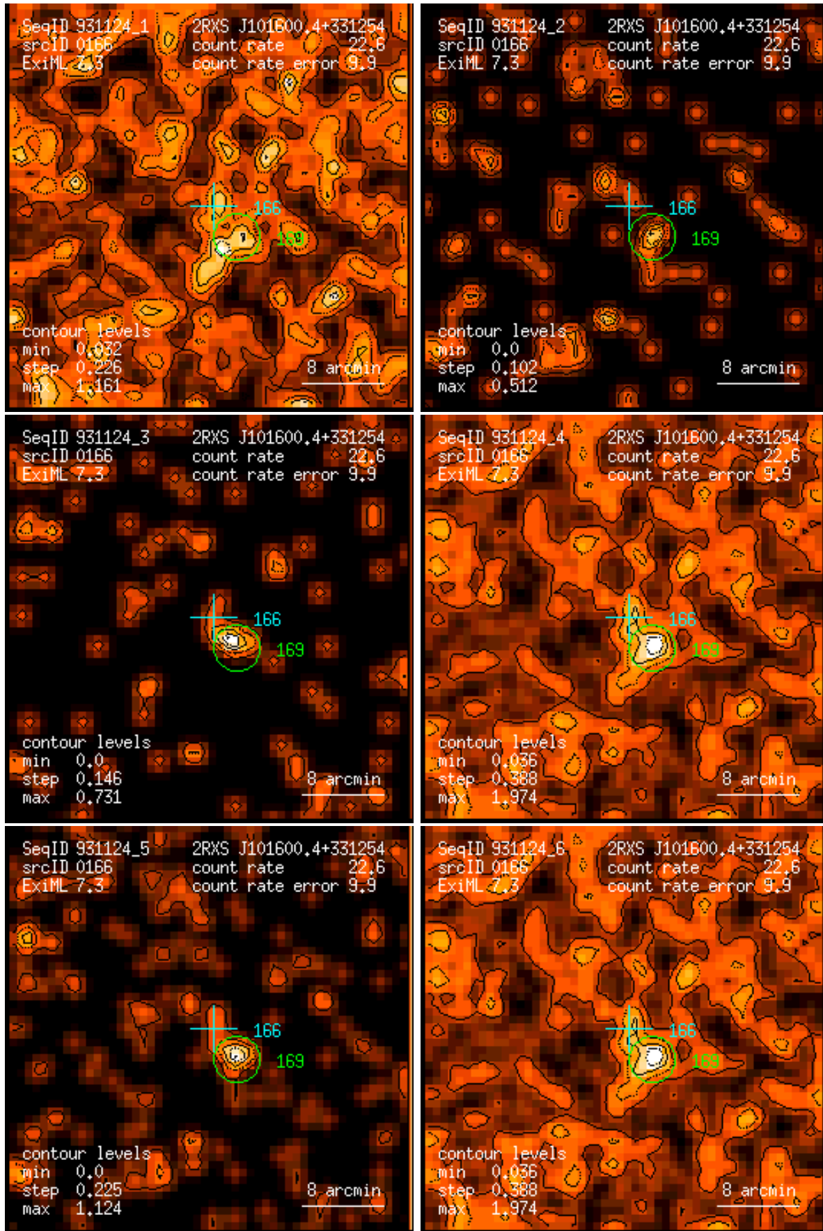
Figure 166: RASS 931124: detection 0166: band rate images, Gaussian filter: (1) PSPC channels 11 – 41, (2) 52 – 90, (3) 91 – 201, (4) 11 – 235, (5) 52 – 201, (6) 11 – 201. Broad band rates in counts/ks. Band rate contour levels in counts/ks/arcmin 2 .
