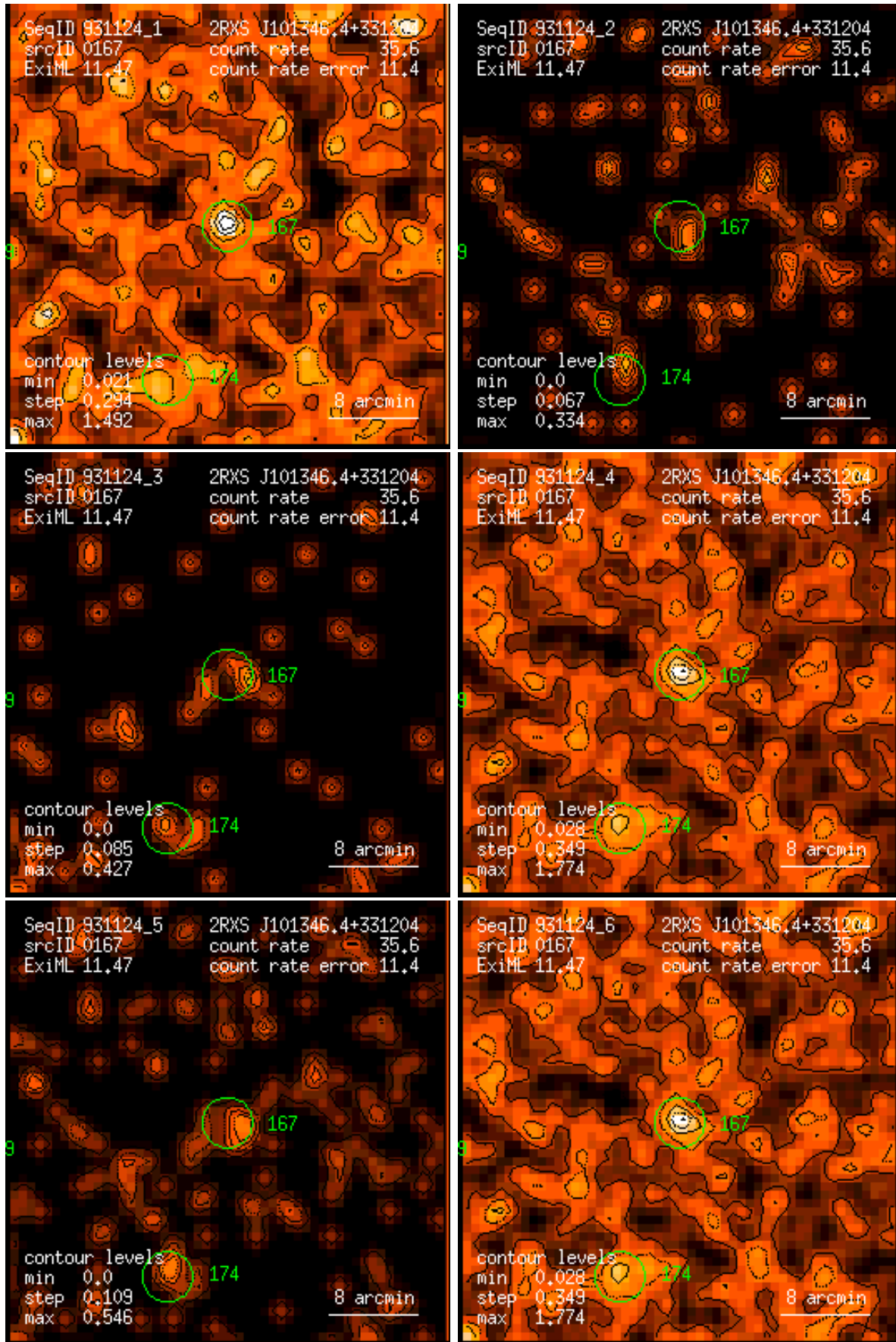
Figure 167: RASS 931124: detection 0167: band rate images, Gaussian filter: (1) PSPC channels 11 – 41, (2) 52 – 90, (3) 91 – 201, (4) 11 – 235, (5) 52 – 201, (6) 11 – 201. Broad band rates in counts/ks. Band rate contour levels in counts/ks/arcmin 2 .
