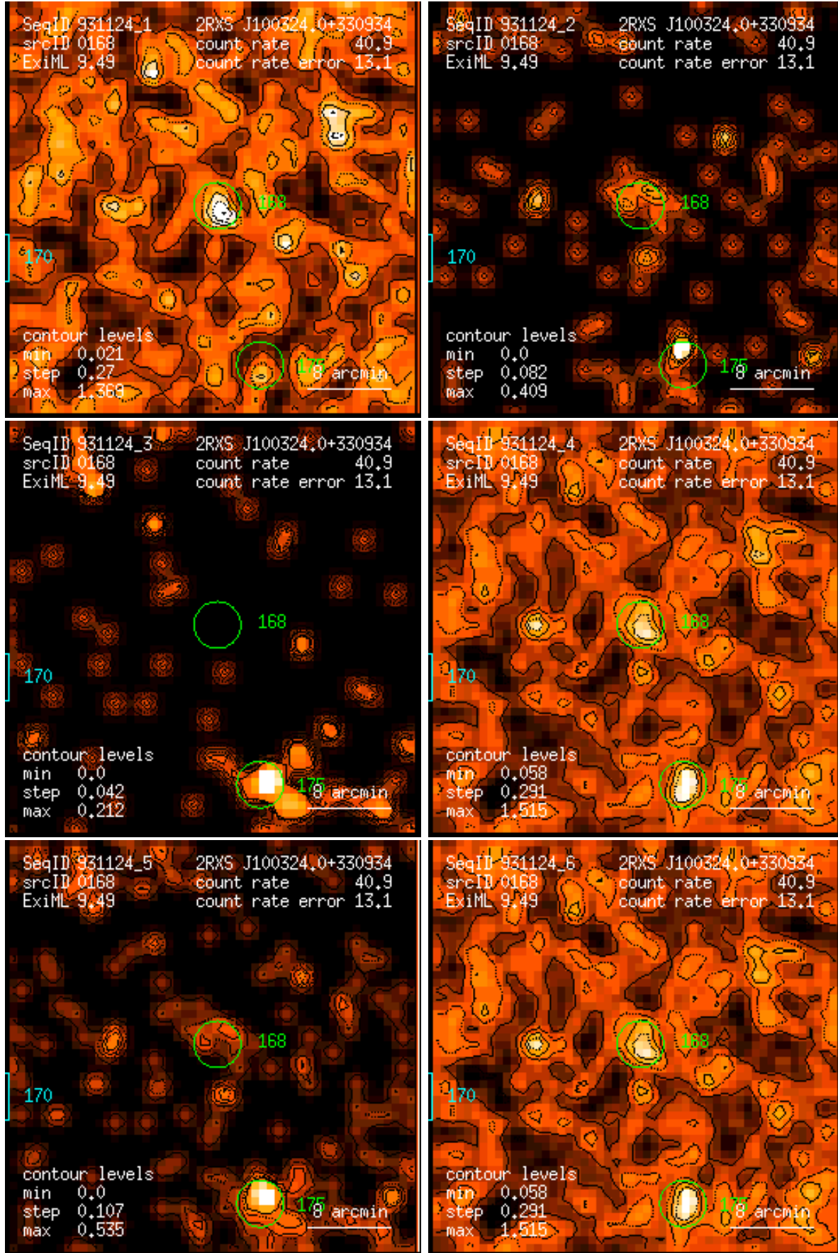
Figure 168: RASS 931124: detection 0168: band rate images, Gaussian filter: (1) PSPC channels 11 – 41, (2) 52 – 90, (3) 91 – 201, (4) 11 – 235, (5) 52 – 201, (6) 11 – 201. Broad band rates in counts/ks. Band rate contour levels in counts/ks/arcmin 2 .
