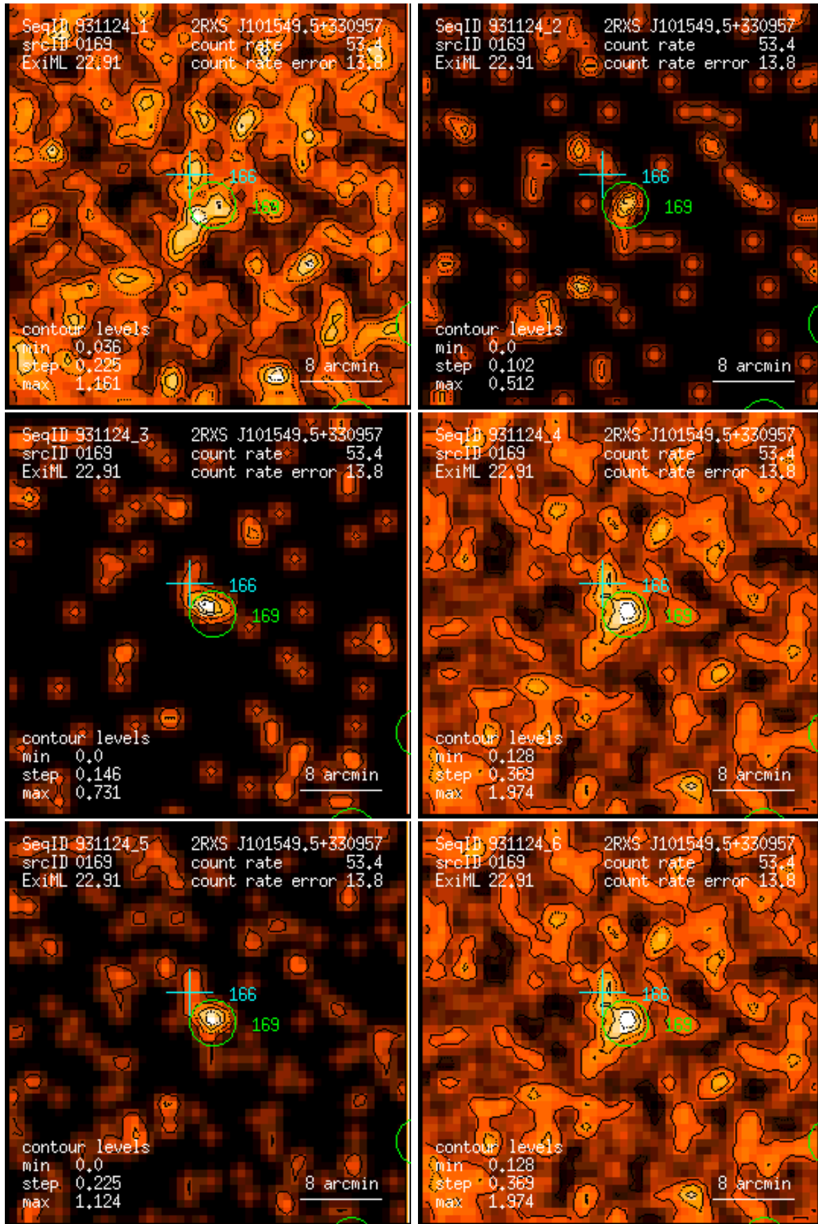
Figure 169: RASS 931124: detection 0169: band rate images, Gaussian filter: (1) PSPC channels 11 – 41, (2) 52 – 90, (3) 91 – 201, (4) 11 – 235, (5) 52 – 201, (6) 11 – 201. Broad band rates in counts/ks. Band rate contour levels in counts/ks/arcmin 2 .
