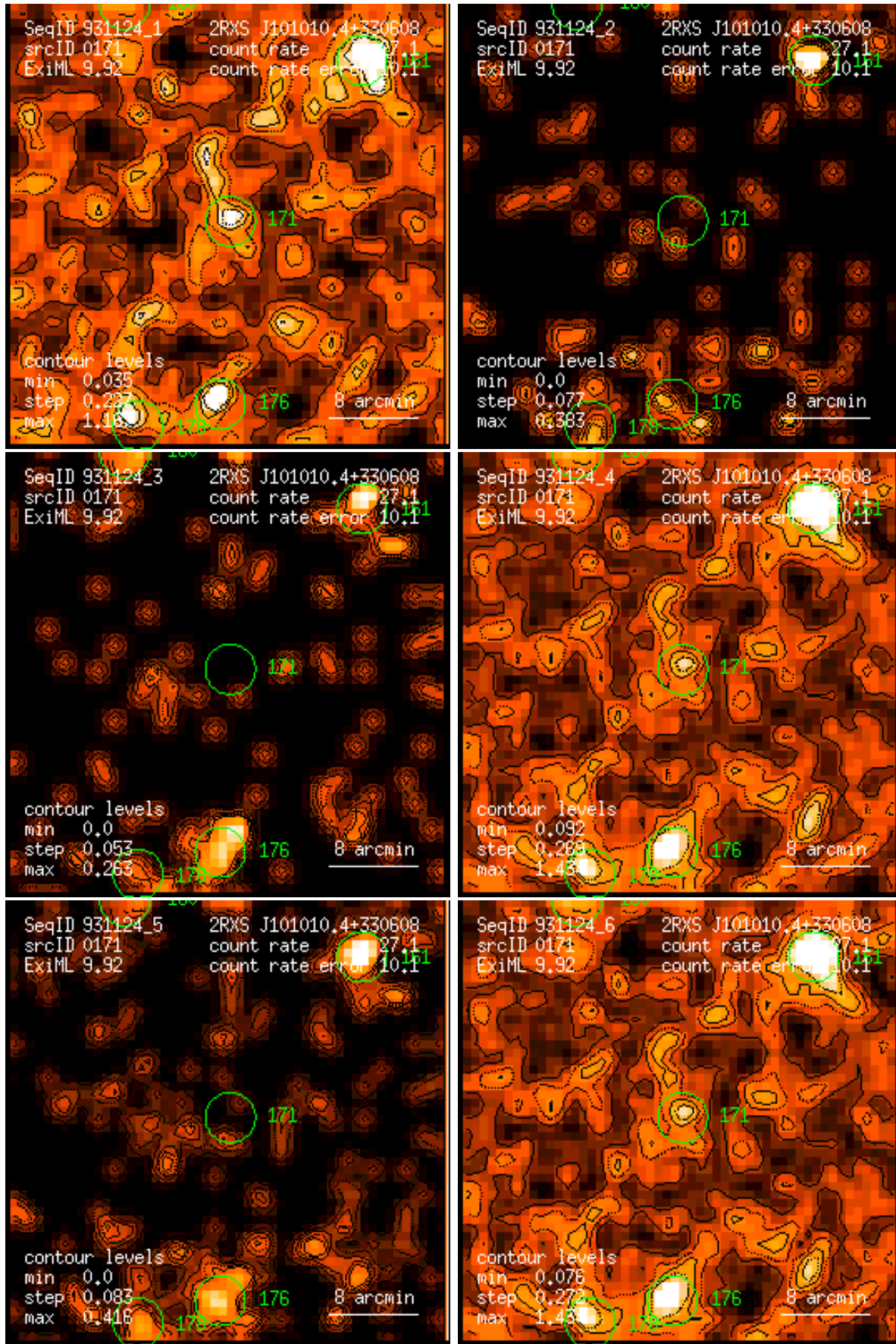
Figure 171: RASS 931124: detection 0171: band rate images, Gaussian filter: (1) PSPC channels 11 – 41, (2) 52 – 90, (3) 91 – 201, (4) 11 – 235, (5) 52 – 201, (6) 11 – 201. Broad band rates in counts/ks. Band rate contour levels in counts/ks/arcmin 2 .
