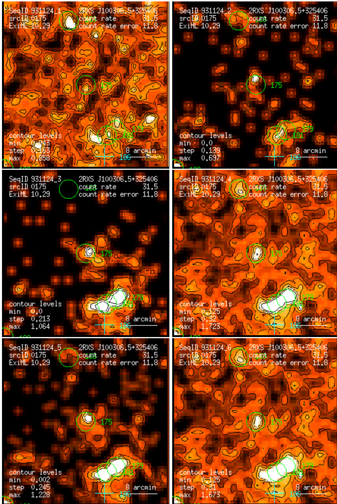
Figure 175: RASS 931124: detection 0175: band rate images, Gaussian filter: (1) PSPC channels 11 – 41, (2) 52 – 90, (3) 91 – 201, (4) 11 – 235, (5) 52 – 201, (6) 11 – 201. Broad band rates in counts/ks. Band rate contour levels in counts/ks/arcmin 2 .
