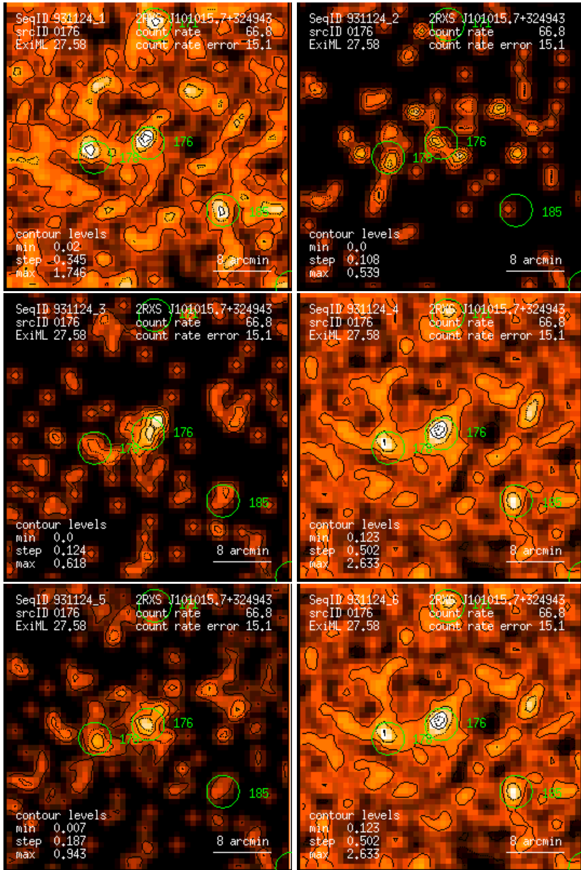
Figure 176: RASS 931124: detection 0176: band rate images, Gaussian filter: (1) PSPC channels 11 – 41, (2) 52 – 90, (3) 91 – 201, (4) 11 – 235, (5) 52 – 201, (6) 11 – 201. Broad band rates in counts/ks. Band rate contour levels in counts/ks/arcmin 2 .
