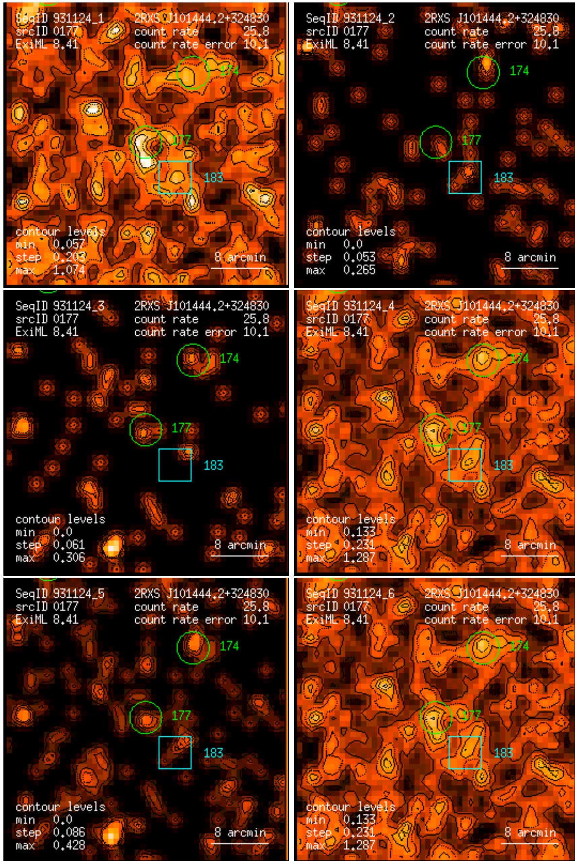
Figure 177: RASS 931124: detection 0177: band rate images, Gaussian filter: (1) PSPC channels 11 – 41, (2) 52 – 90, (3) 91 – 201, (4) 11 – 235, (5) 52 – 201, (6) 11 – 201. Broad band rates in counts/ks. Band rate contour levels in counts/ks/arcmin 2 .
