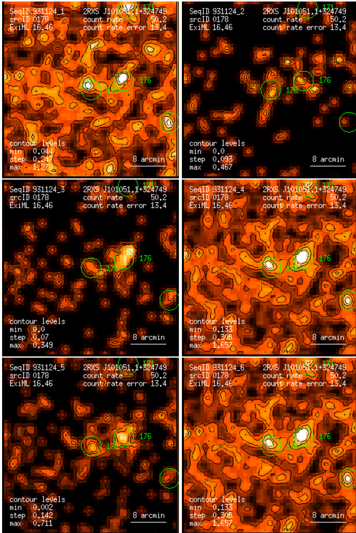
Figure 178: RASS 931124: detection 0178: band rate images, Gaussian filter: (1) PSPC channels 11 – 41, (2) 52 – 90, (3) 91 – 201, (4) 11 – 235, (5) 52 – 201, (6) 11 – 201. Broad band rates in counts/ks. Band rate contour levels in counts/ks/arcmin 2 .
