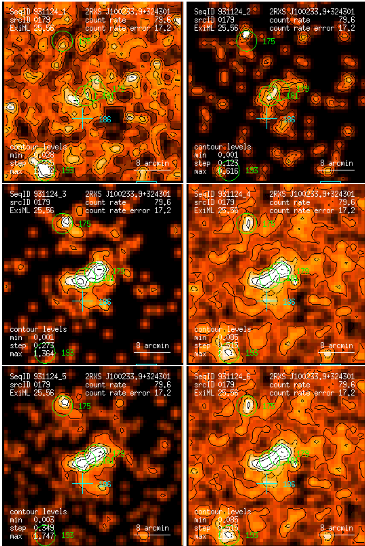
Figure 179: RASS 931124: detection 0179: band rate images, Gaussian filter: (1) PSPC channels 11 – 41, (2) 52 – 90, (3) 91 – 201, (4) 11 – 235, (5) 52 – 201, (6) 11 – 201. Broad band rates in counts/ks. Band rate contour levels in counts/ks/arcmin 2 .
