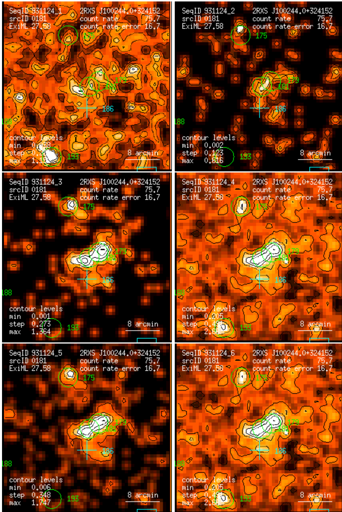
Figure 181: RASS 931124: detection 0181: band rate images, Gaussian filter: (1) PSPC channels 11 – 41, (2) 52 – 90, (3) 91 – 201, (4) 11 – 235, (5) 52 – 201, (6) 11 – 201. Broad band rates in counts/ks. Band rate contour levels in counts/ks/arcmin 2 .
