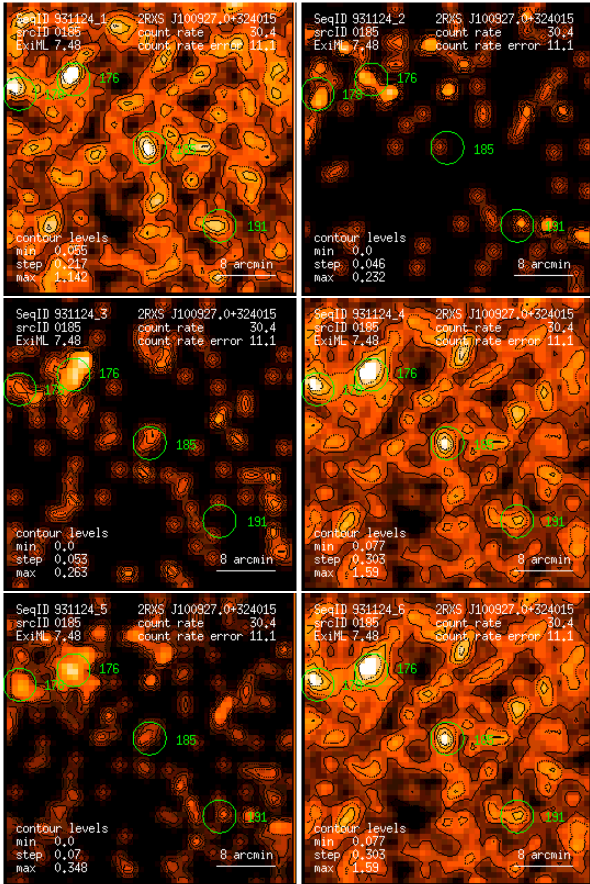
Figure 185: RASS 931124: detection 0185: band rate images, Gaussian filter: (1) PSPC channels 11 – 41, (2) 52 – 90, (3) 91 – 201, (4) 11 – 235, (5) 52 – 201, (6) 11 – 201. Broad band rates in counts/ks. Band rate contour levels in counts/ks/arcmin 2 .
