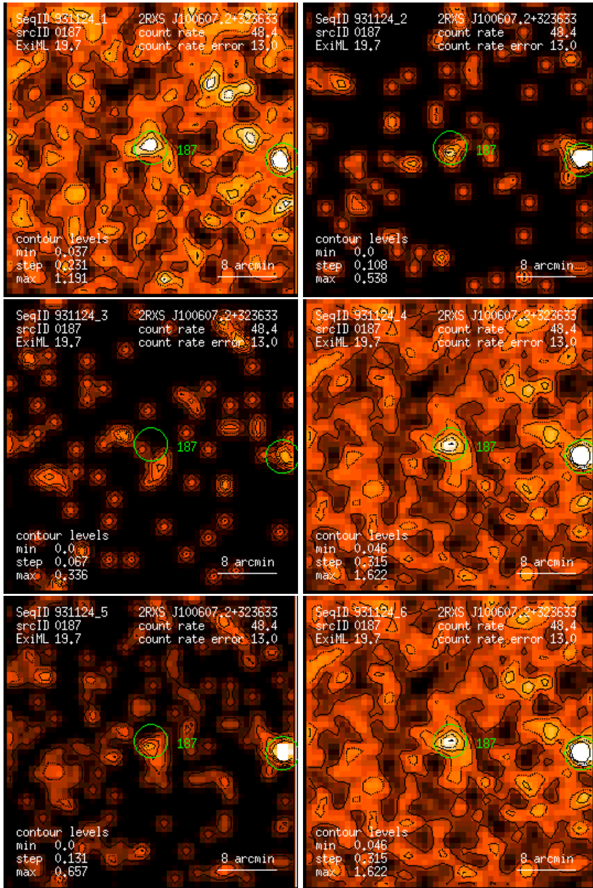
Figure 187: RASS 931124: detection 0187: band rate images, Gaussian filter: (1) PSPC channels 11 – 41, (2) 52 – 90, (3) 91 – 201, (4) 11 – 235, (5) 52 – 201, (6) 11 – 201. Broad band rates in counts/ks. Band rate contour levels in counts/ks/arcmin 2 .
