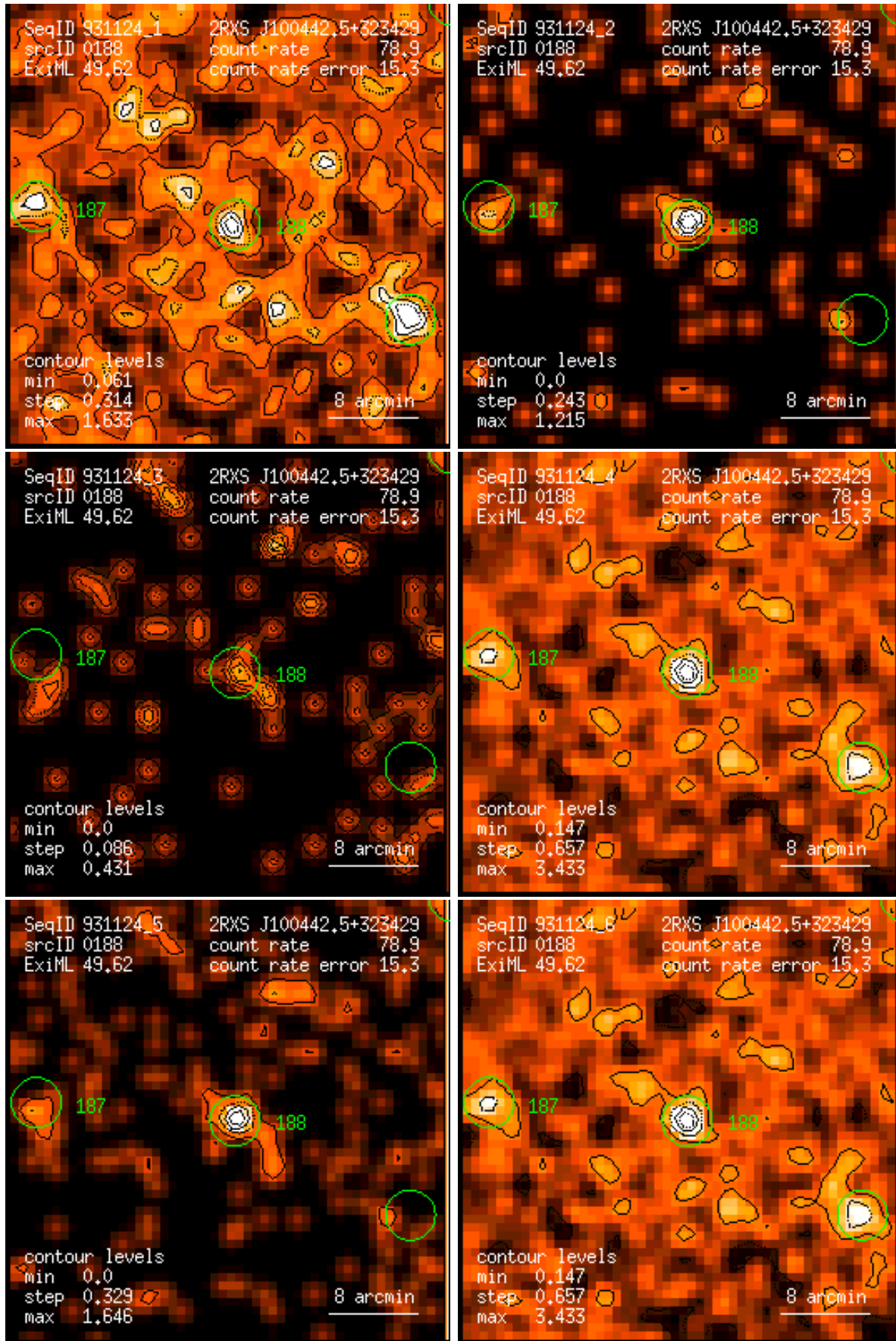
Figure 188: RASS 931124: detection 0188: band rate images, Gaussian filter: (1) PSPC channels 11 – 41, (2) 52 – 90, (3) 91 – 201, (4) 11 – 235, (5) 52 – 201, (6) 11 – 201. Broad band rates in counts/ks. Band rate contour levels in counts/ks/arcmin 2 .
