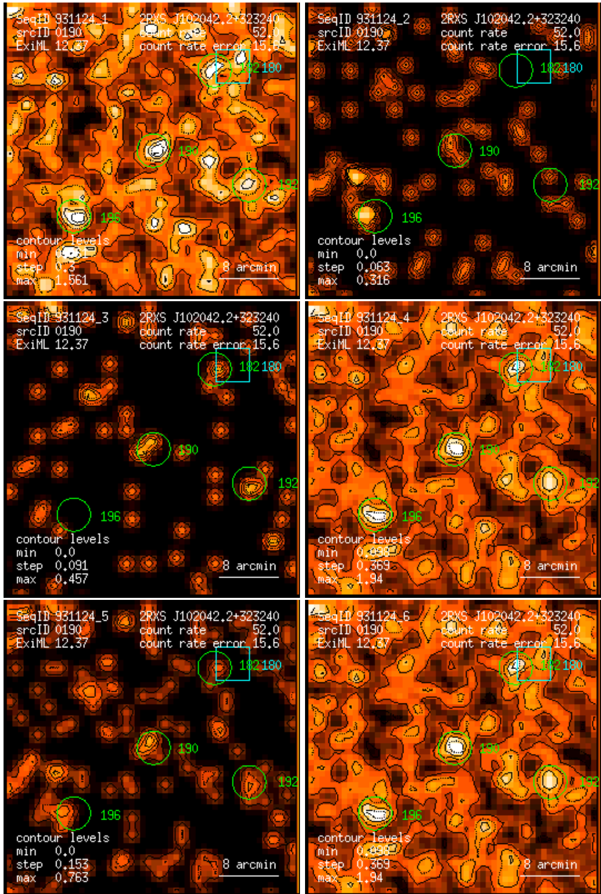
Figure 190: RASS 931124: detection 0190: band rate images, Gaussian filter: (1) PSPC channels 11 – 41, (2) 52 – 90, (3) 91 – 201, (4) 11 – 235, (5) 52 – 201, (6) 11 – 201. Broad band rates in counts/ks. Band rate contour levels in counts/ks/arcmin 2 .
