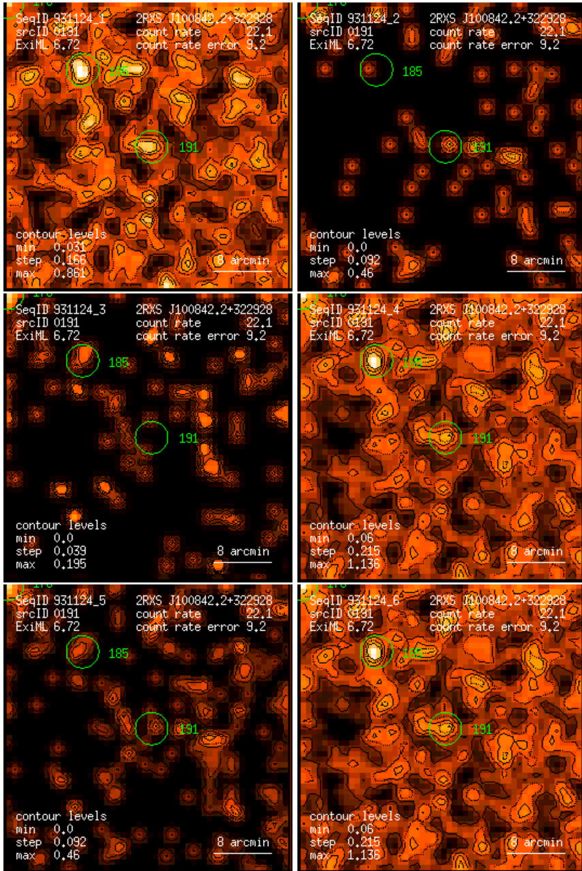
Figure 191: RASS 931124: detection 0191: band rate images, Gaussian filter: (1) PSPC channels 11 – 41, (2) 52 – 90, (3) 91 – 201, (4) 11 – 235, (5) 52 – 201, (6) 11 – 201. Broad band rates in counts/ks. Band rate contour levels in counts/ks/arcmin 2 .
