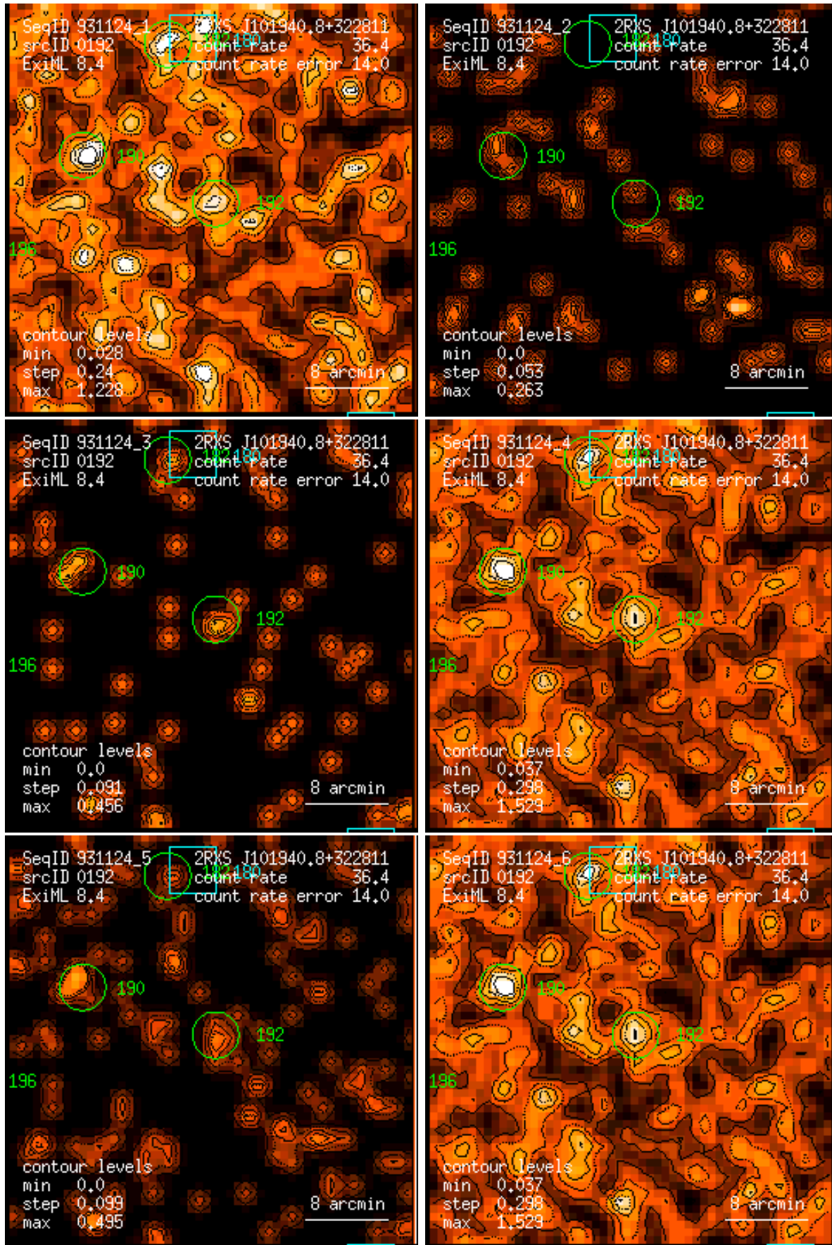
Figure 192: RASS 931124: detection 0192: band rate images, Gaussian filter: (1) PSPC channels 11 – 41, (2) 52 – 90, (3) 91 – 201, (4) 11 – 235, (5) 52 – 201, (6) 11 – 201. Broad band rates in counts/ks. Band rate contour levels in counts/ks/arcmin 2 .
