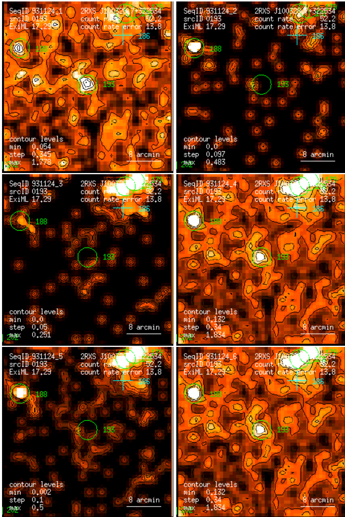
Figure 193: RASS 931124: detection 0193: band rate images, Gaussian filter: (1) PSPC channels 11 – 41, (2) 52 – 90, (3) 91 – 201, (4) 11 – 235, (5) 52 – 201, (6) 11 – 201. Broad band rates in counts/ks. Band rate contour levels in counts/ks/arcmin 2 .
