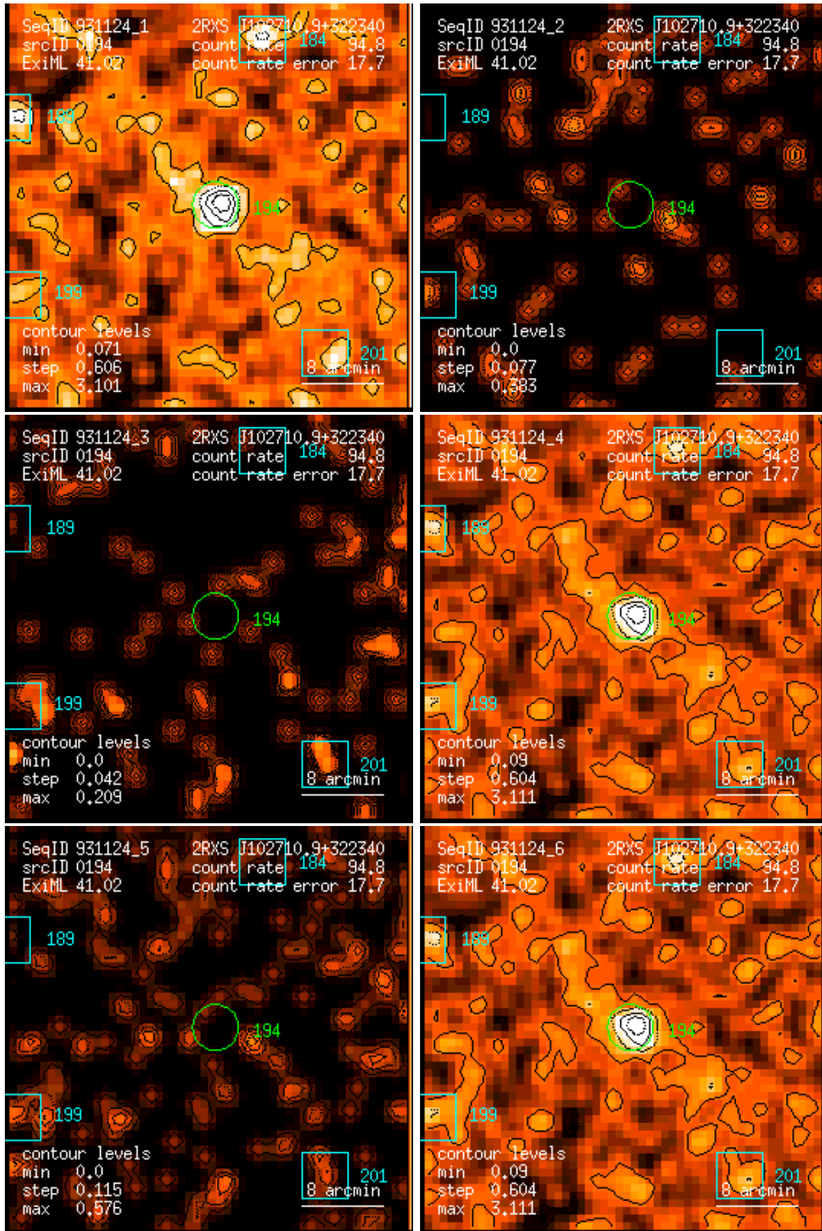
Figure 194: RASS 931124: detection 0194: band rate images, Gaussian filter: (1) PSPC channels 11 – 41, (2) 52 – 90, (3) 91 – 201, (4) 11 – 235, (5) 52 – 201, (6) 11 – 201. Broad band rates in counts/ks. Band rate contour levels in counts/ks/arcmin 2 .
