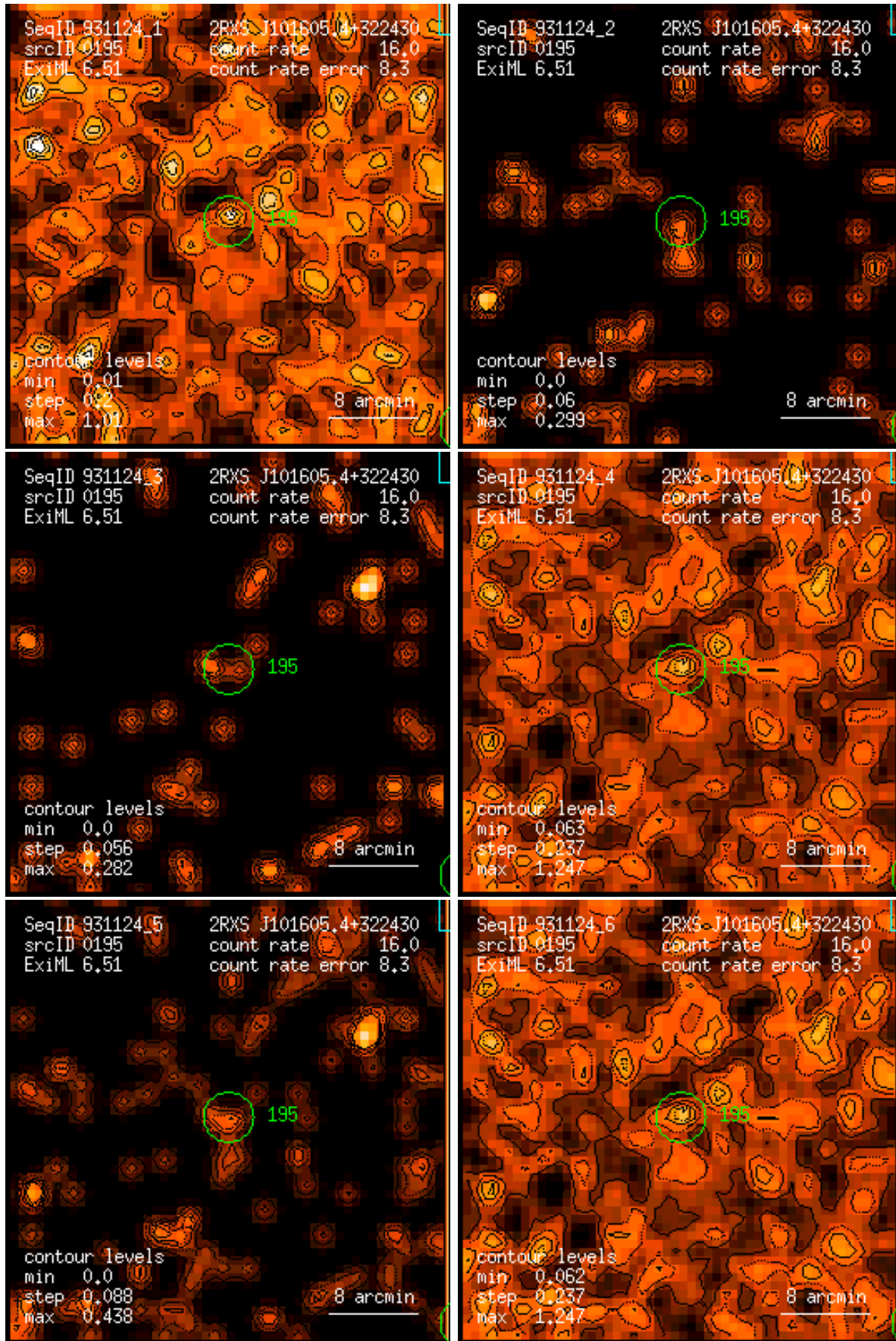
Figure 195: RASS 931124: detection 0195: band rate images, Gaussian filter: (1) PSPC channels 11 – 41, (2) 52 – 90, (3) 91 – 201, (4) 11 – 235, (5) 52 – 201, (6) 11 – 201. Broad band rates in counts/ks. Band rate contour levels in counts/ks/arcmin 2 .
