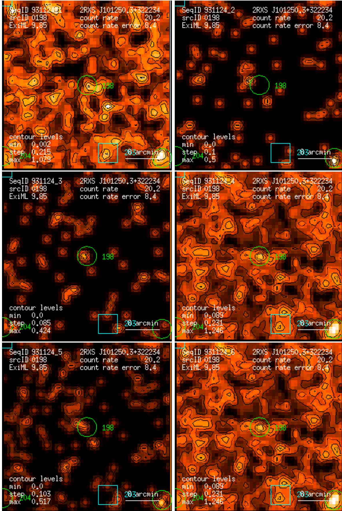
Figure 198: RASS 931124: detection 0198: band rate images, Gaussian filter: (1) PSPC channels 11 – 41, (2) 52 – 90, (3) 91 – 201, (4) 11 – 235, (5) 52 – 201, (6) 11 – 201. Broad band rates in counts/ks. Band rate contour levels in counts/ks/arcmin 2 .
