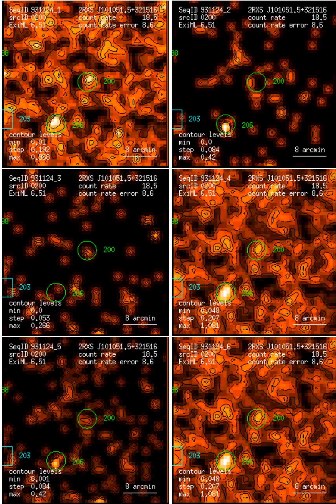
Figure 200: RASS 931124: detection 0200: band rate images, Gaussian filter: (1) PSPC channels 11 – 41, (2) 52 – 90, (3) 91 – 201, (4) 11 – 235, (5) 52 – 201, (6) 11 – 201. Broad band rates in counts/ks. Band rate contour levels in counts/ks/arcmin 2 .
