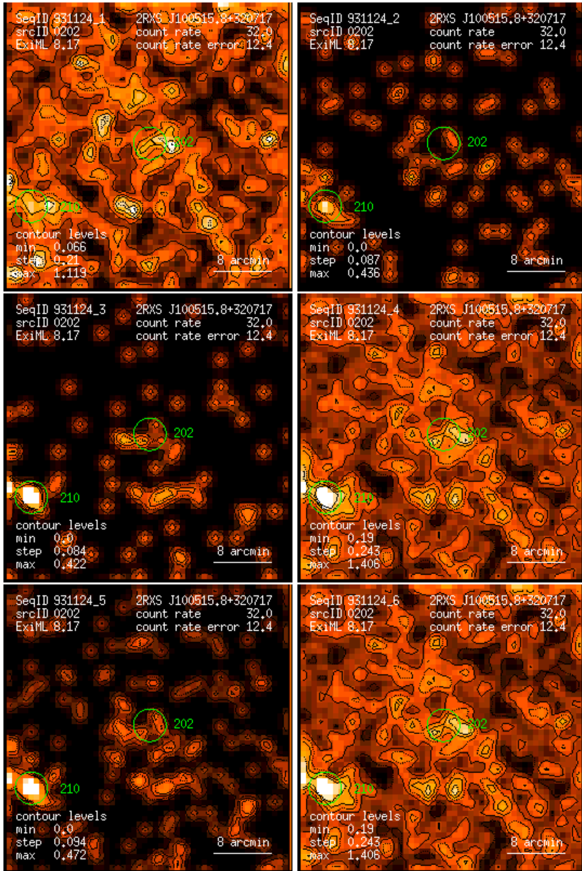
Figure 202: RASS 931124: detection 0202: band rate images, Gaussian filter: (1) PSPC channels 11 – 41, (2) 52 – 90, (3) 91 – 201, (4) 11 – 235, (5) 52 – 201, (6) 11 – 201. Broad band rates in counts/ks. Band rate contour levels in counts/ks/arcmin 2 .
