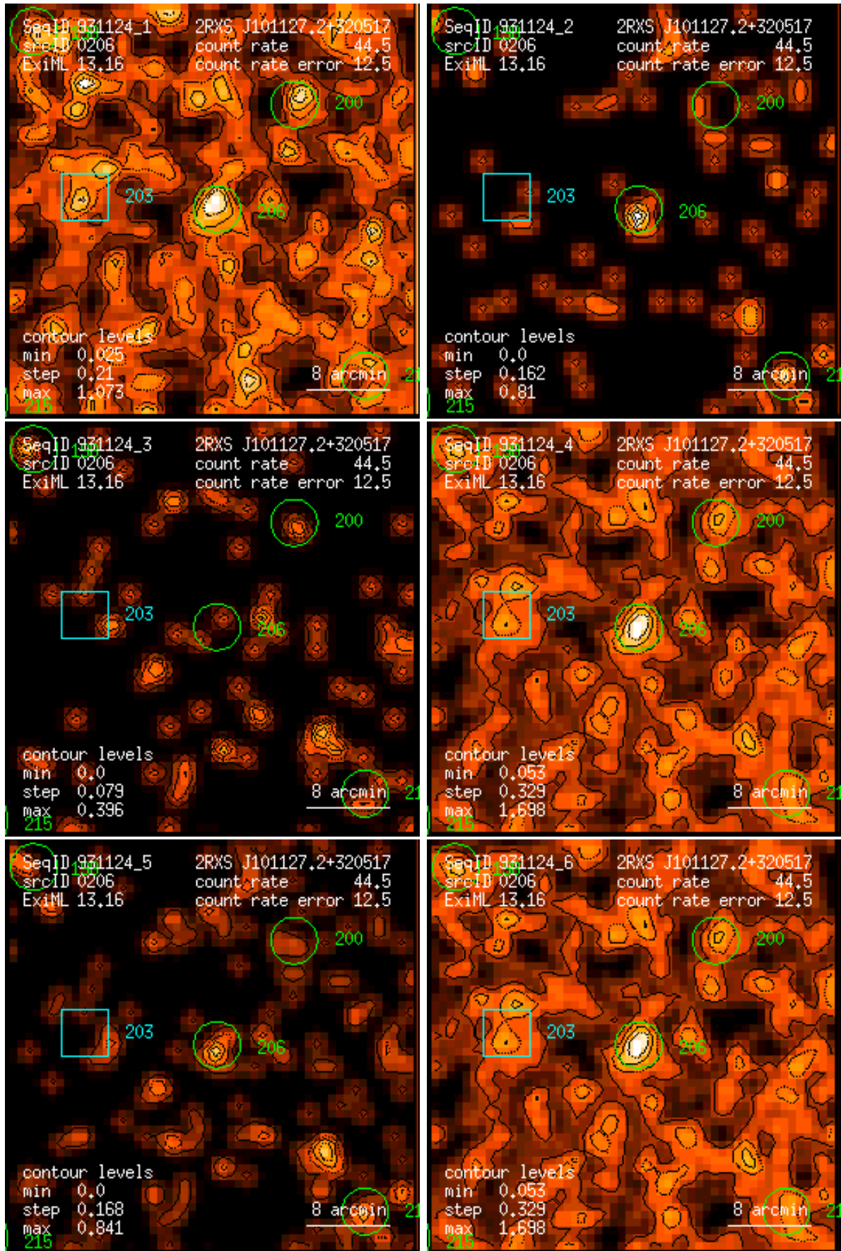
Figure 206: RASS 931124: detection 0206: band rate images, Gaussian filter: (1) PSPC channels 11 – 41, (2) 52 – 90, (3) 91 – 201, (4) 11 – 235, (5) 52 – 201, (6) 11 – 201. Broad band rates in counts/ks. Band rate contour levels in counts/ks/arcmin 2 .
