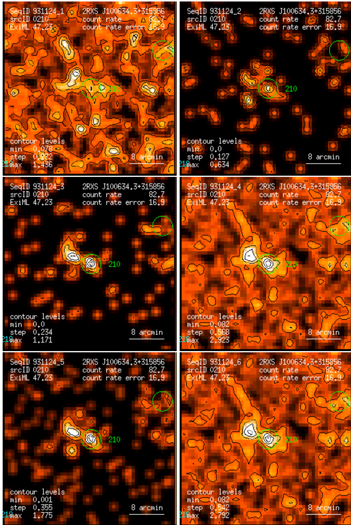
Figure 210: RASS 931124: detection 0210: band rate images, Gaussian filter: (1) PSPC channels 11 – 41, (2) 52 – 90, (3) 91 – 201, (4) 11 – 235, (5) 52 – 201, (6) 11 – 201. Broad band rates in counts/ks. Band rate contour levels in counts/ks/arcmin 2 .
