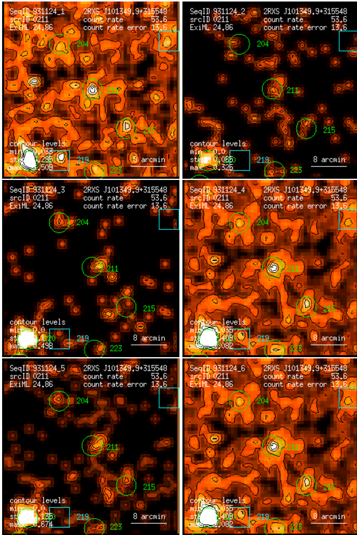
Figure 211: RASS 931124: detection 0211: band rate images, Gaussian filter: (1) PSPC channels 11 – 41, (2) 52 – 90, (3) 91 – 201, (4) 11 – 235, (5) 52 – 201, (6) 11 – 201. Broad band rates in counts/ks. Band rate contour levels in counts/ks/arcmin 2 .
