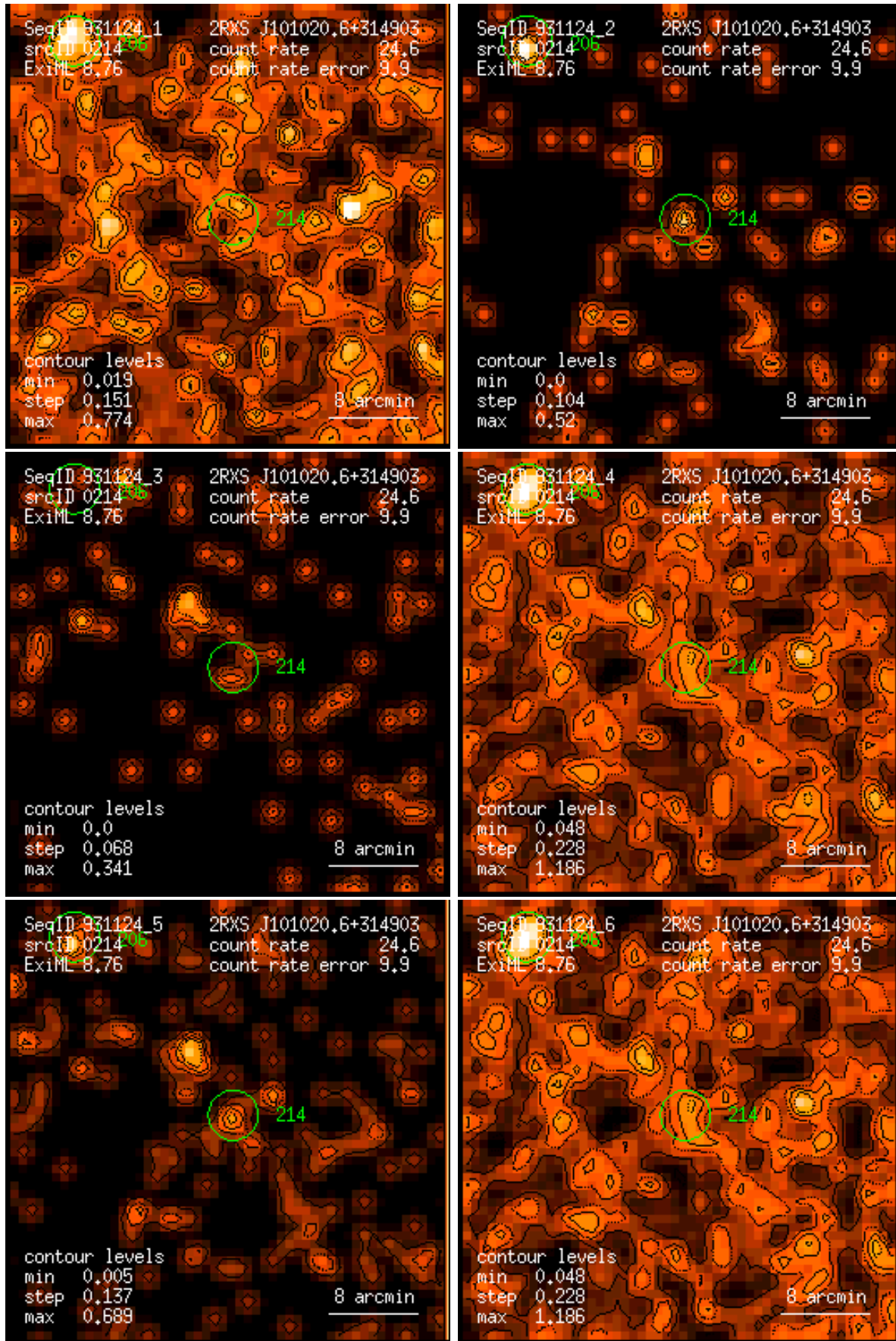
Figure 214: RASS 931124: detection 0214: band rate images, Gaussian filter: (1) PSPC channels 11 – 41, (2) 52 – 90, (3) 91 – 201, (4) 11 – 235, (5) 52 – 201, (6) 11 – 201. Broad band rates in counts/ks. Band rate contour levels in counts/ks/arcmin 2 .
