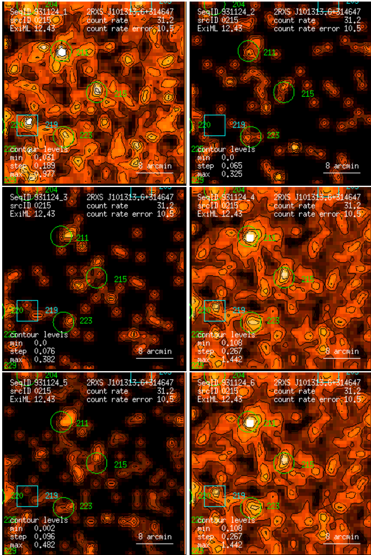
Figure 215: RASS 931124: detection 0215: band rate images, Gaussian filter: (1) PSPC channels 11 – 41, (2) 52 – 90, (3) 91 – 201, (4) 11 – 235, (5) 52 – 201, (6) 11 – 201. Broad band rates in counts/ks. Band rate contour levels in counts/ks/arcmin 2 .
