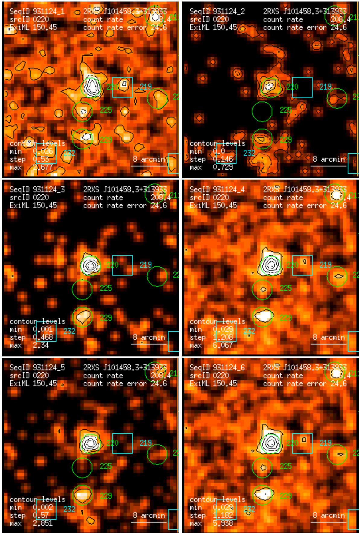
Figure 220: RASS 931124: detection 0220: band rate images, Gaussian filter: (1) PSPC channels 11 – 41, (2) 52 – 90, (3) 91 – 201, (4) 11 – 235, (5) 52 – 201, (6) 11 – 201. Broad band rates in counts/ks. Band rate contour levels in counts/ks/arcmin 2 .
