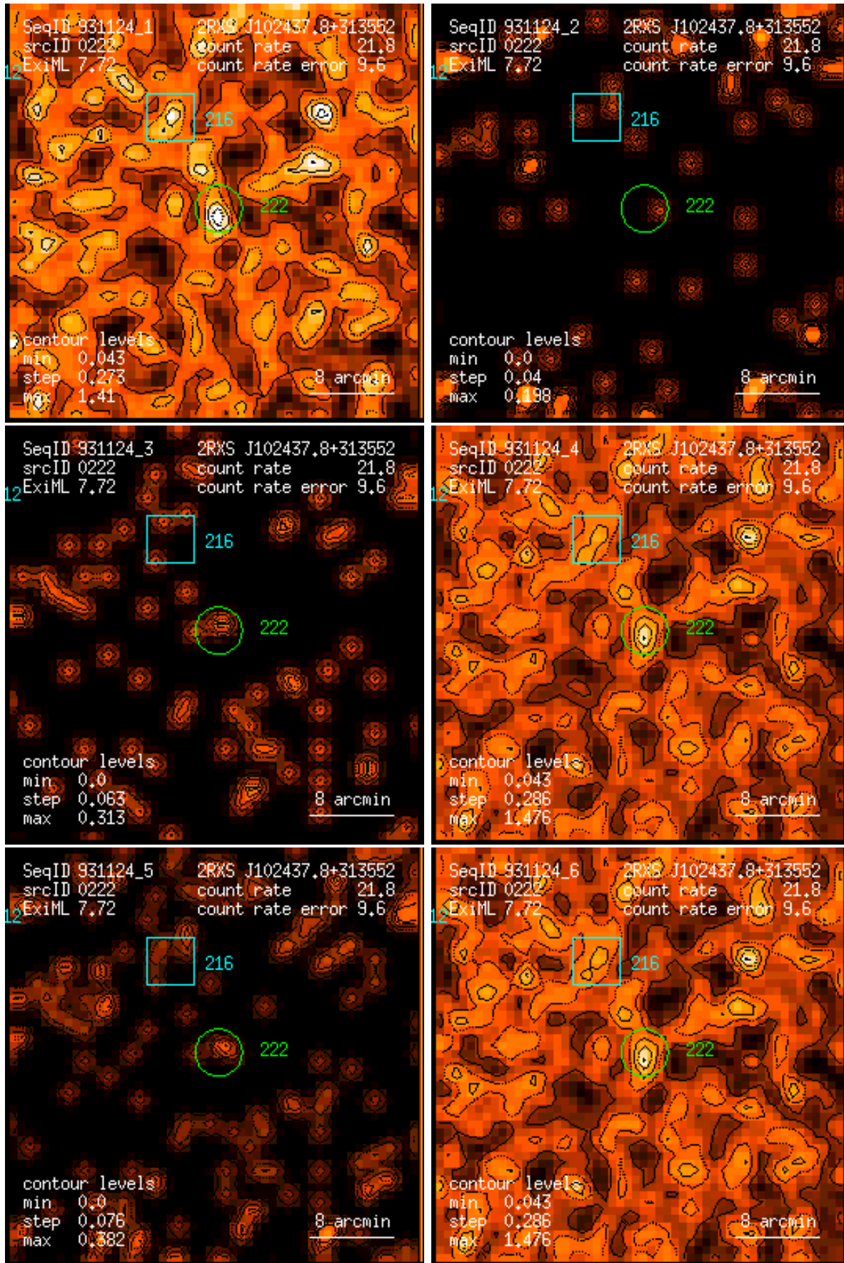
Figure 222: RASS 931124: detection 0222: band rate images, Gaussian filter: (1) PSPC channels 11 – 41, (2) 52 – 90, (3) 91 – 201, (4) 11 – 235, (5) 52 – 201, (6) 11 – 201. Broad band rates in counts/ks. Band rate contour levels in counts/ks/arcmin 2 .
