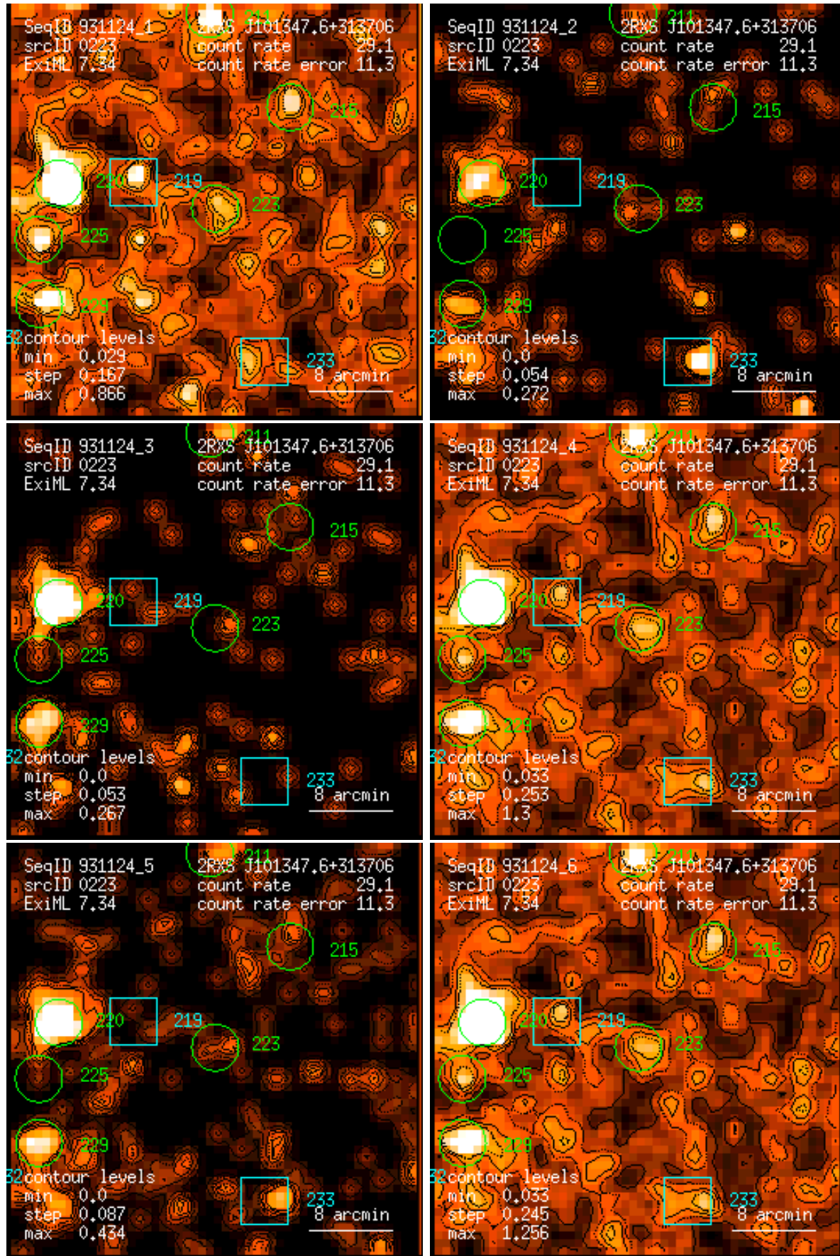
Figure 223: RASS 931124: detection 0223: band rate images, Gaussian filter: (1) PSPC channels 11 – 41, (2) 52 – 90, (3) 91 – 201, (4) 11 – 235, (5) 52 – 201, (6) 11 – 201. Broad band rates in counts/ks. Band rate contour levels in counts/ks/arcmin 2 .
