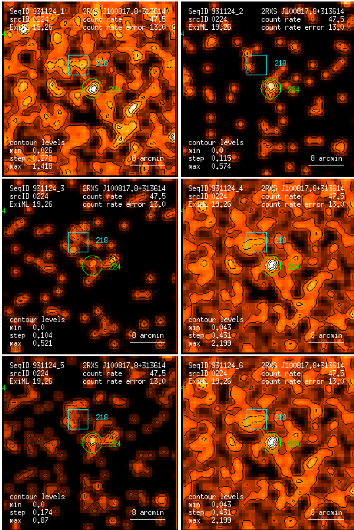
Figure 224: RASS 931124: detection 0224: band rate images, Gaussian filter: (1) PSPC channels 11 – 41, (2) 52 – 90, (3) 91 – 201, (4) 11 – 235, (5) 52 – 201, (6) 11 – 201. Broad band rates in counts/ks. Band rate contour levels in counts/ks/arcmin 2 .
