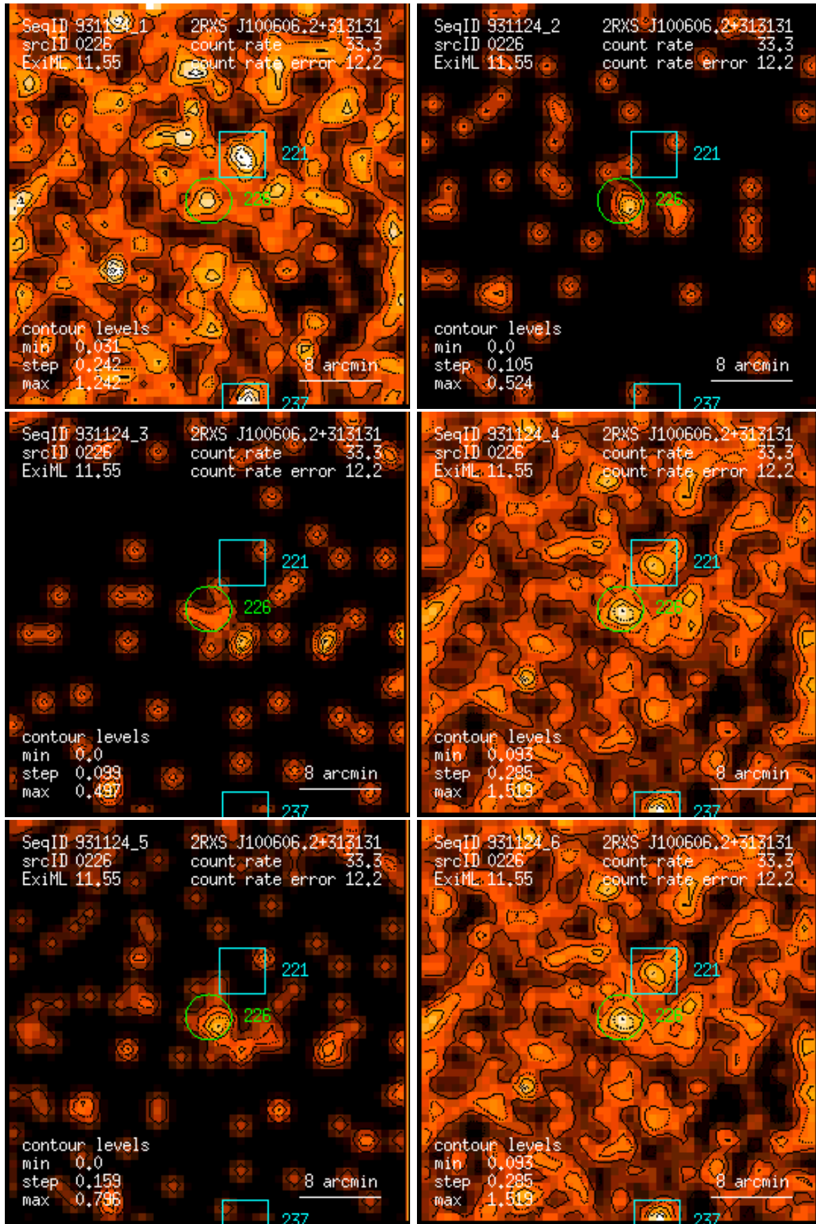
Figure 226: RASS 931124: detection 0226: band rate images, Gaussian filter: (1) PSPC channels 11 – 41, (2) 52 – 90, (3) 91 – 201, (4) 11 – 235, (5) 52 – 201, (6) 11 – 201. Broad band rates in counts/ks. Band rate contour levels in counts/ks/arcmin 2 .
